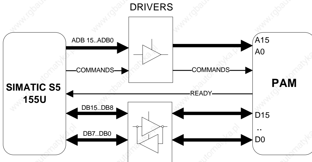
Figure 6: 155U Mode
