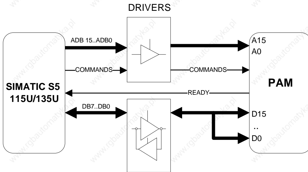
Figure 5: 115U/135U Mode
