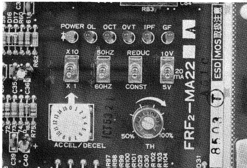
Fig. 15.2.4 Setting Switches
