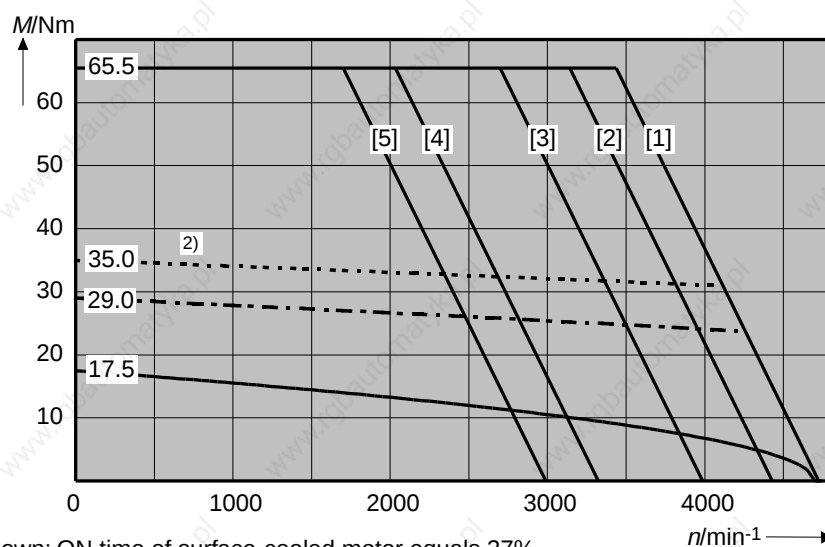
Fig 10.6: Torque-speed characteristics curve MDD 112
