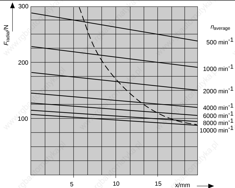
Fig 3.4: Shaft load
