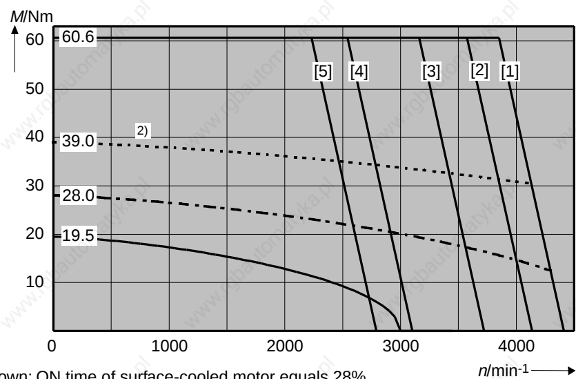
Fig 9.7: Torque-speed characteristics curve - MDD 093
