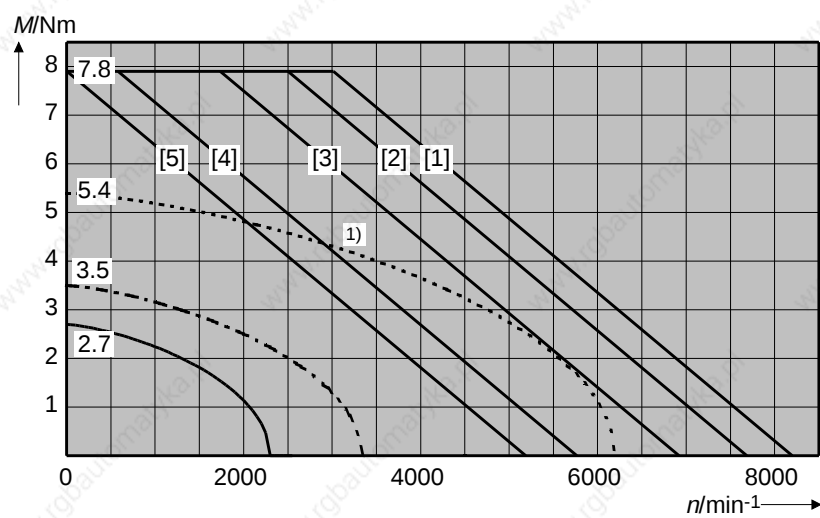
Fig 6.6: Torque-speed characteristics curves - MDD 065
