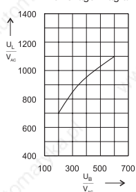
Arc voltage-Diagram
