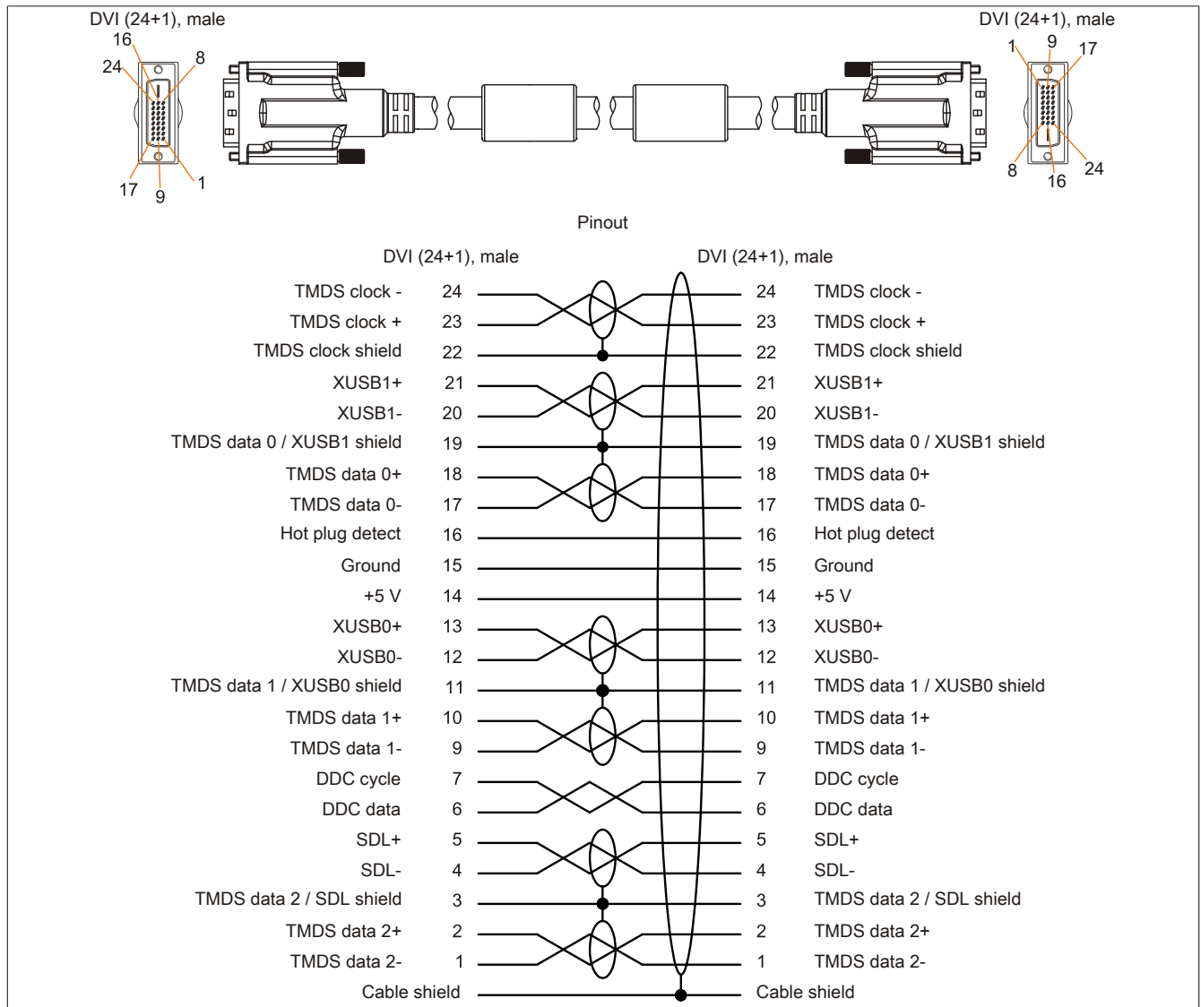
Figure 112: 5CASDL.0xxx-03 - Pinout
