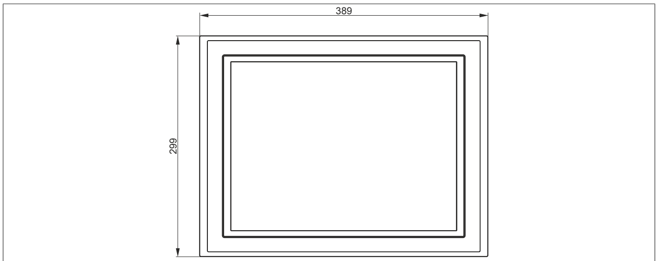
Figure 26: 5AP5120.1505-000 - Dimensions
