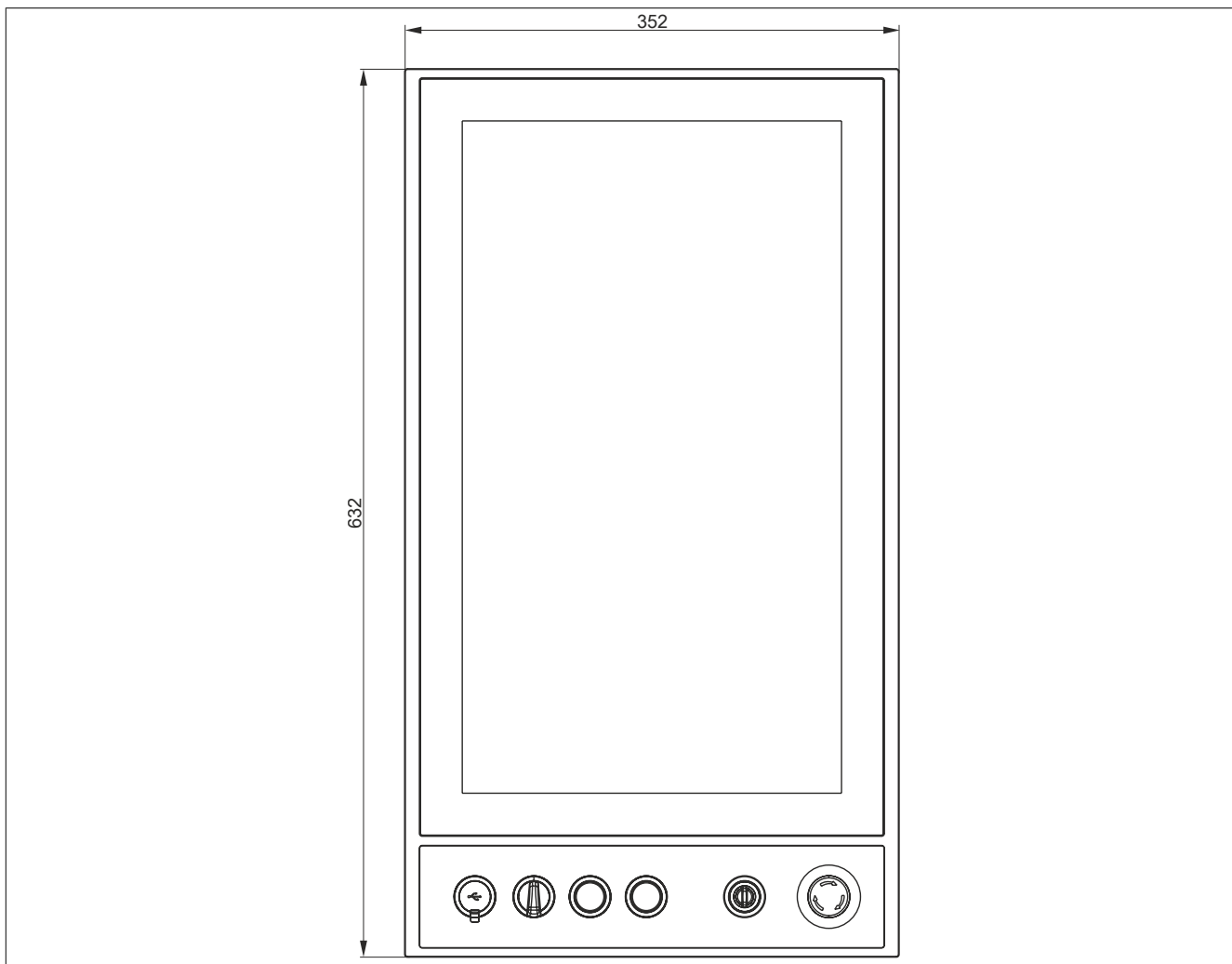
Figure 52: 5AP5230.215I-000 - Dimensions
