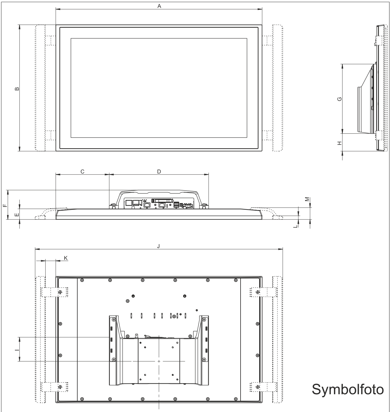
Figure 8: AP5120/AP5130 with 5ACCM01.0100-000 and 5ACCHD0x.xxx-000 - Dimensions
