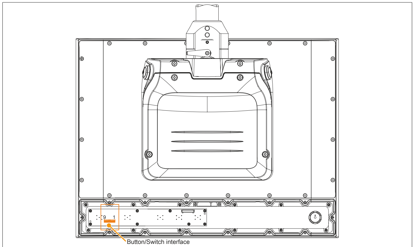
Figure 25: Button/Switch interface
