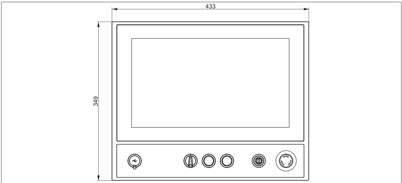
Figure 42: 5AP5230.156B-000 - Dimensions
