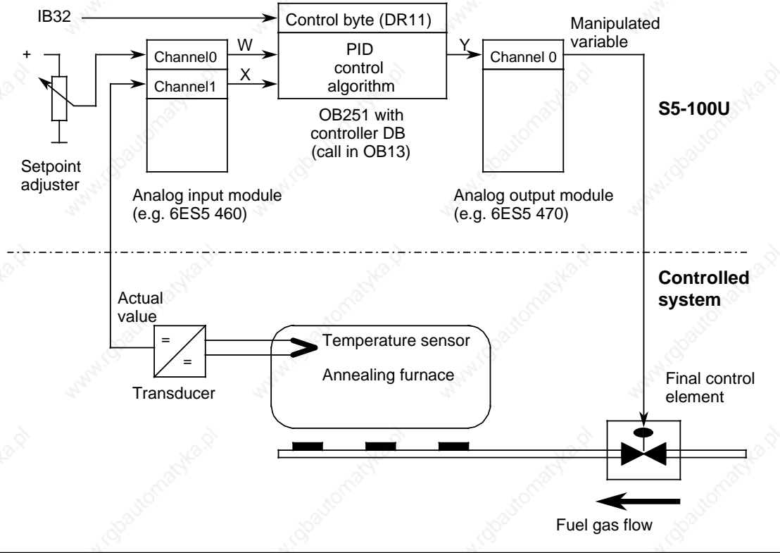
Figure 9-9. Process Schematic
