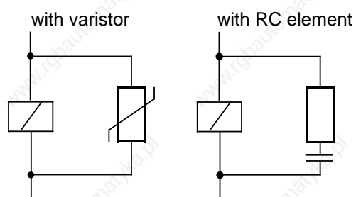
Figure 3-27. Wiring Coils
