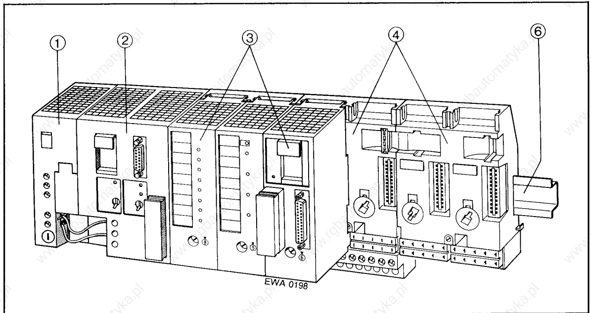
Figure 2-1. The S5-100U
