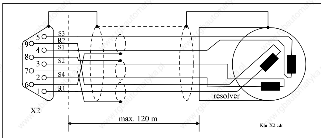
Fig. 54: Resolver interface
