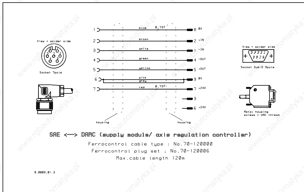
Fig. 13: Absolute value encoder cables
