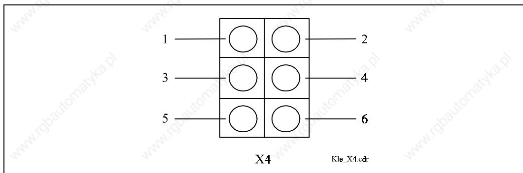
Fig. 55: Measuring points axis regulation controller
