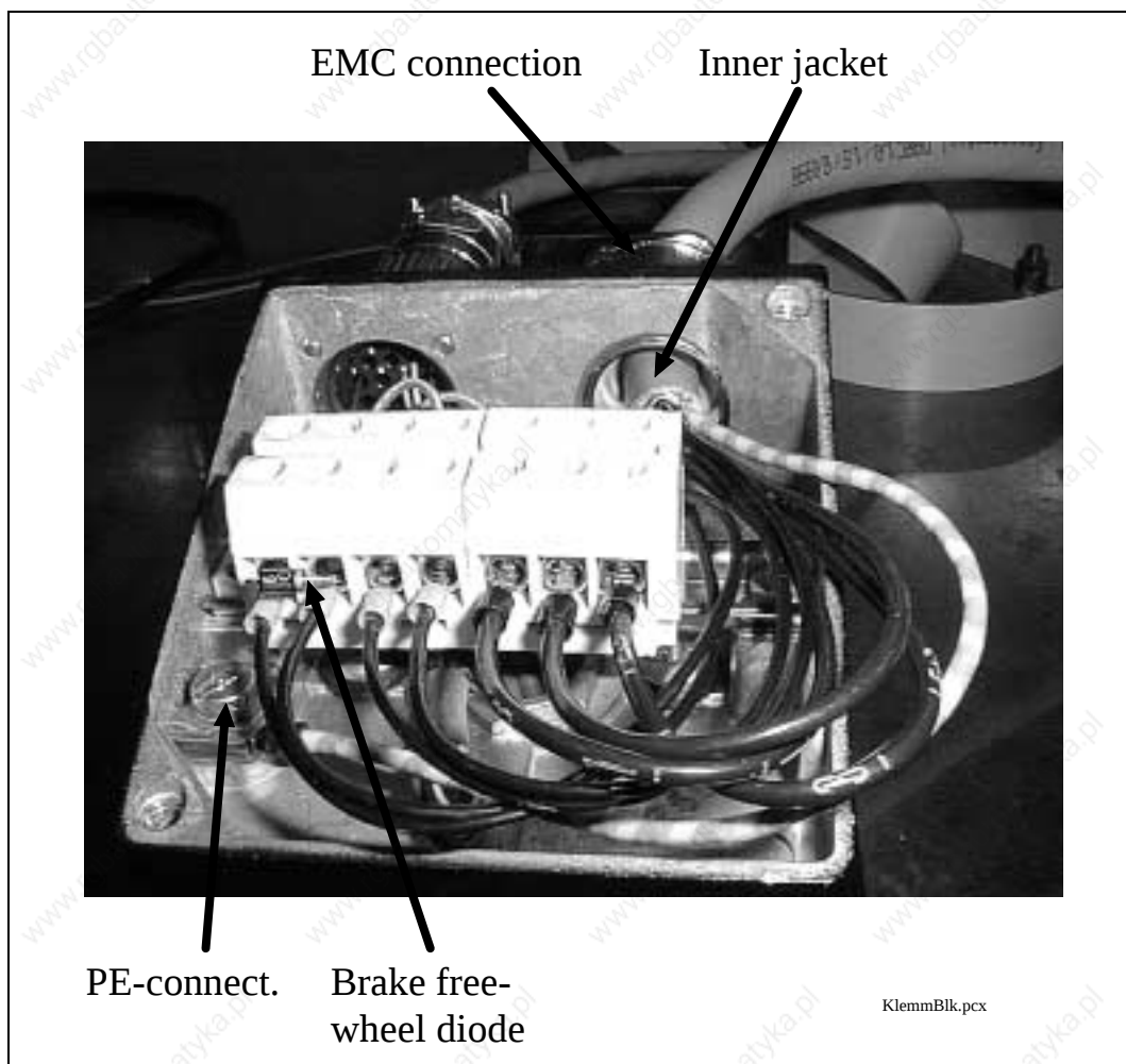
Fig. 25: Detail photo motor terminal board
