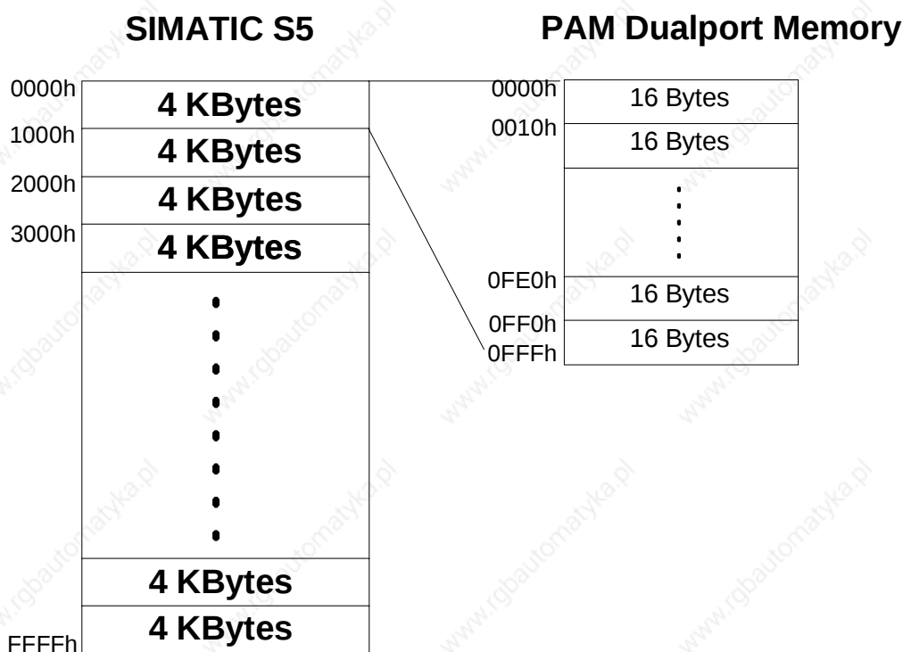
Figure 7: Memory configuration
