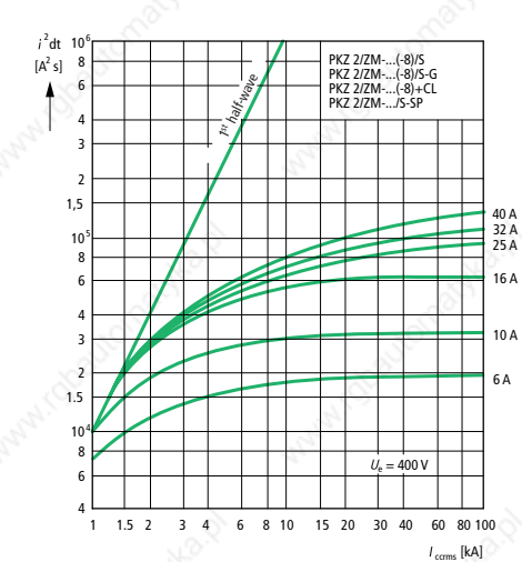
Let-through energy values, motor protector combinations
