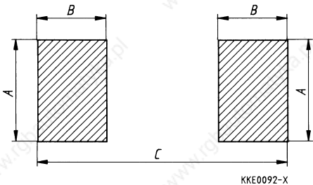
Recommended maximum dimensions (mm)
