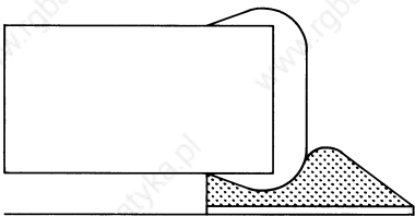
Poor wetting
