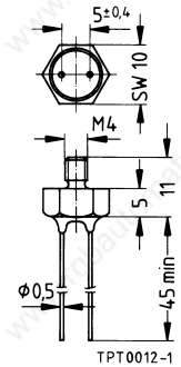
Dimensions (mm)
