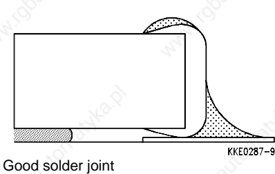
Good solder joint
