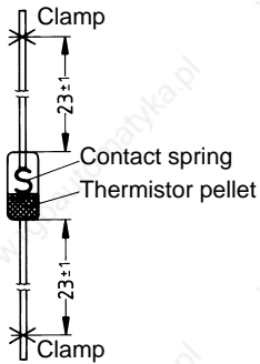
TPT0024-P
