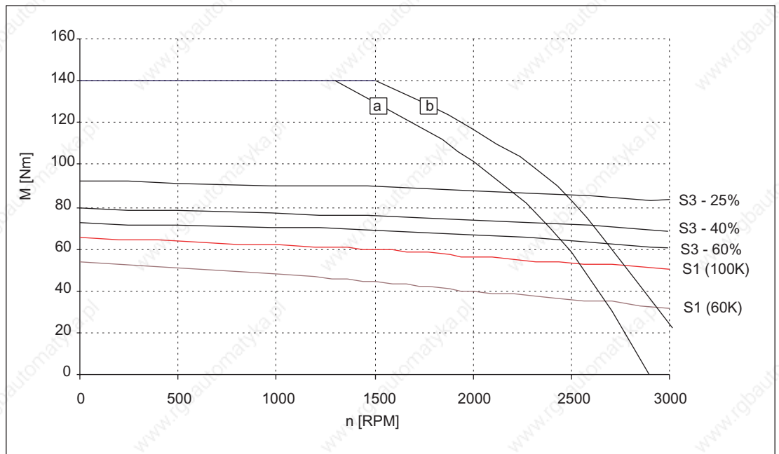
Figure 3-60 Speed-torque diagram 1FT6105-8SC7
