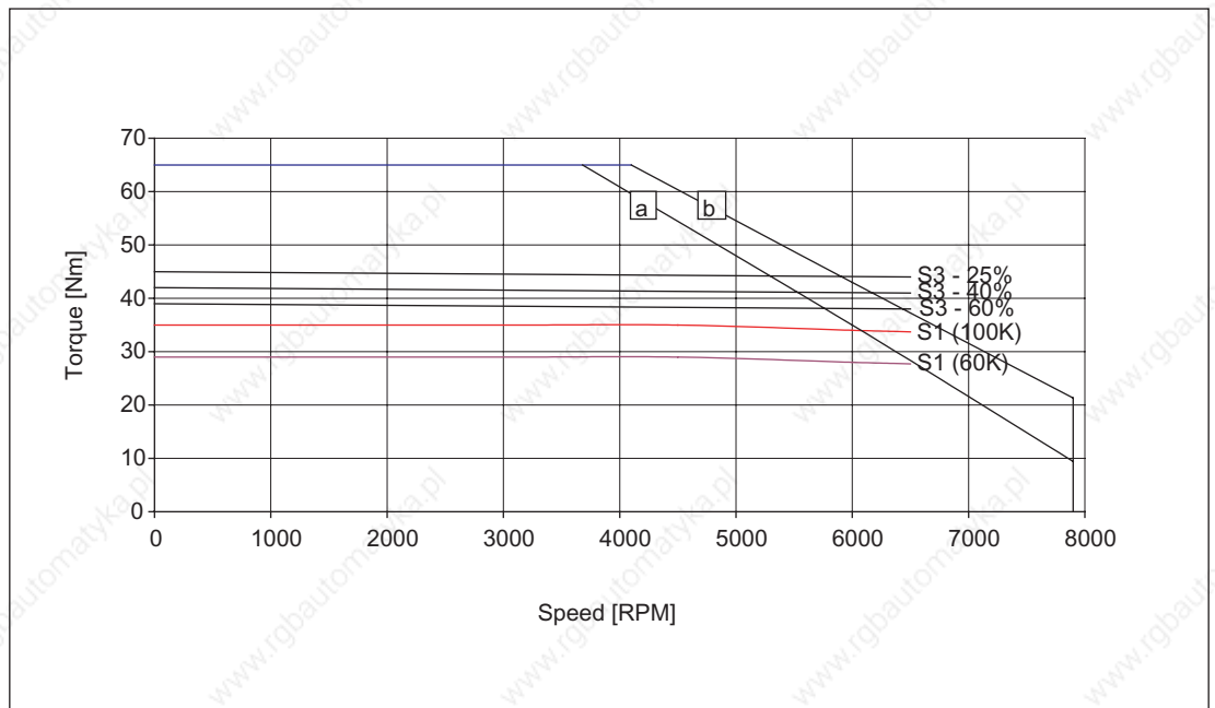
Figure 3-86 Speed-torque diagram 1FT6084-8WK71
