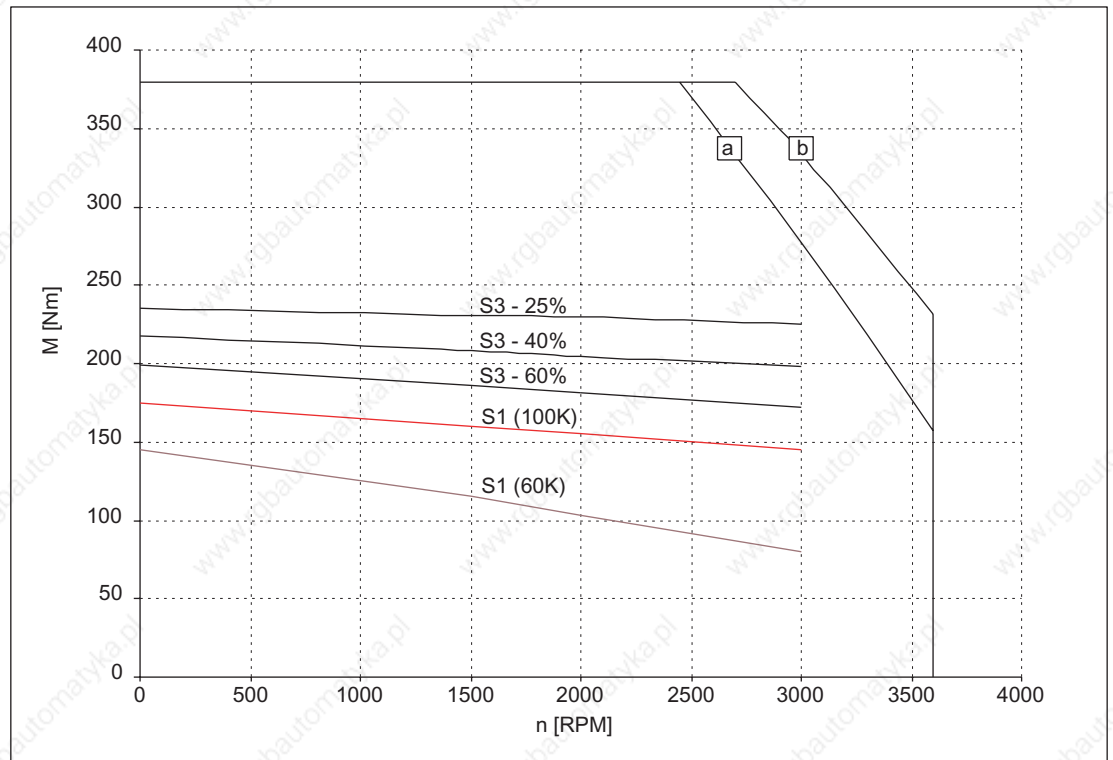
Figure 3-74 Speed-torque diagram 1FT6136-6SF71
