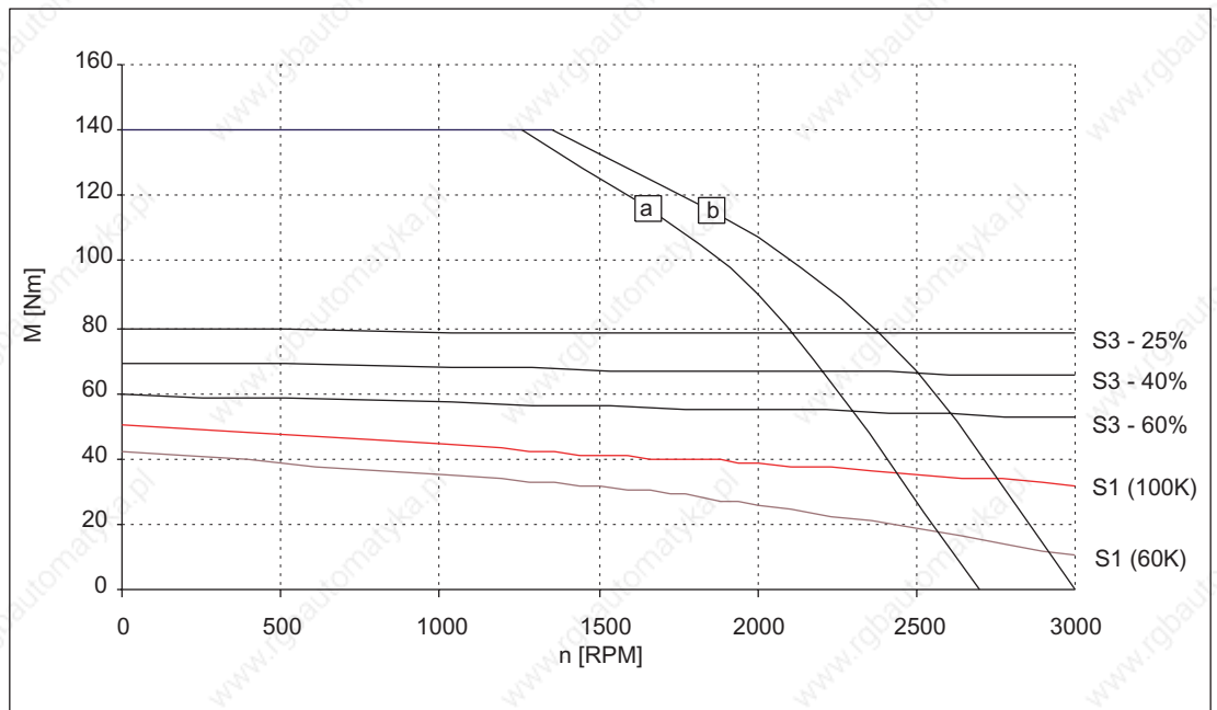
Figure 3-41 Speed-torque diagram 1FT6105-8AC7
