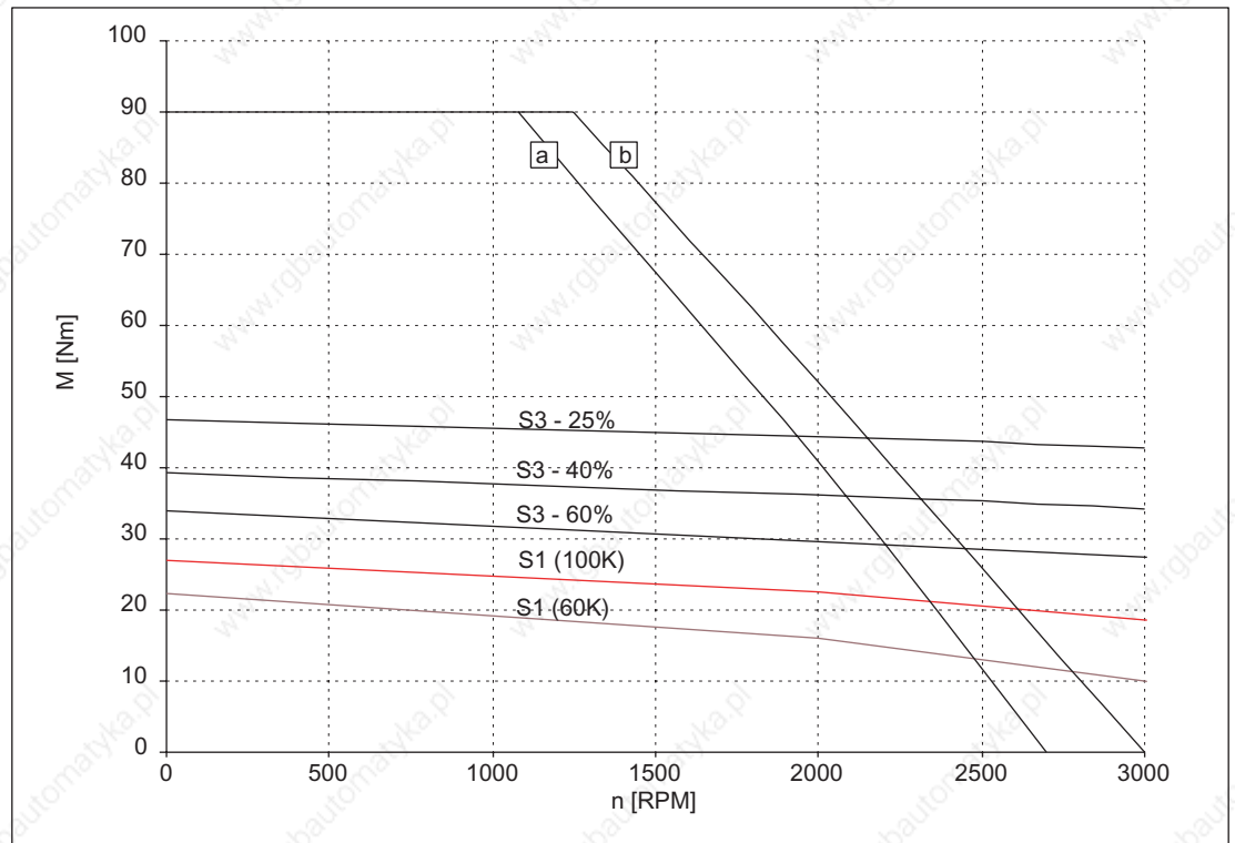
Figure 3-33 Speed-torque diagram 1FT6086-8AC7□
