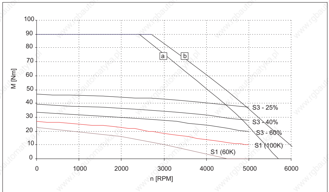
Figure 3-35 Speed-torque diagram 1FT6086-□AH7□
