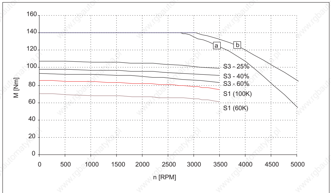
Figure 3-91 Speed-torque diagram 1FT6105-8WF7□
