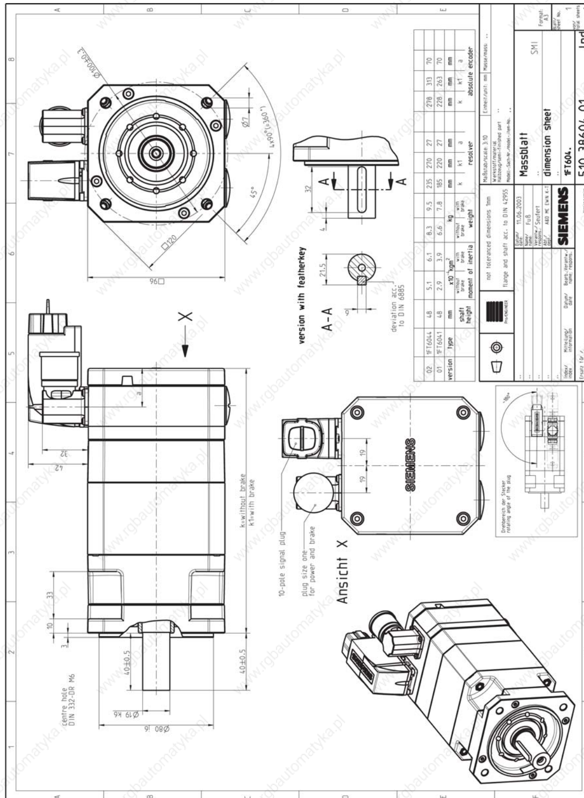
Figure 5-3 1FT604□-□A□DQ
