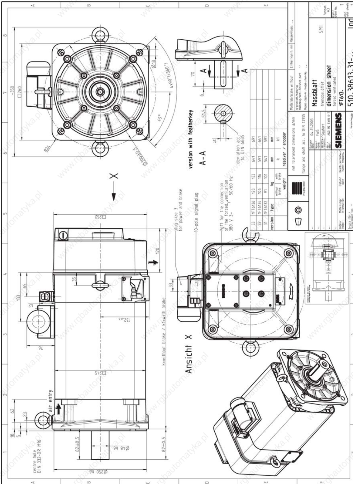
Figure 5-11 1FT613□-□S□plug□DQ
