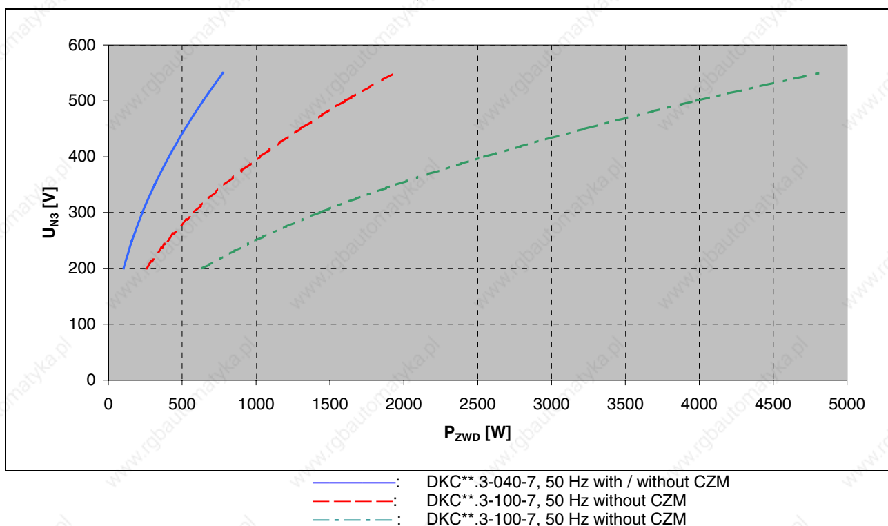
Fig. 4-36: Allowed DC bus continuous power in single-phase mode with 50 Hz
