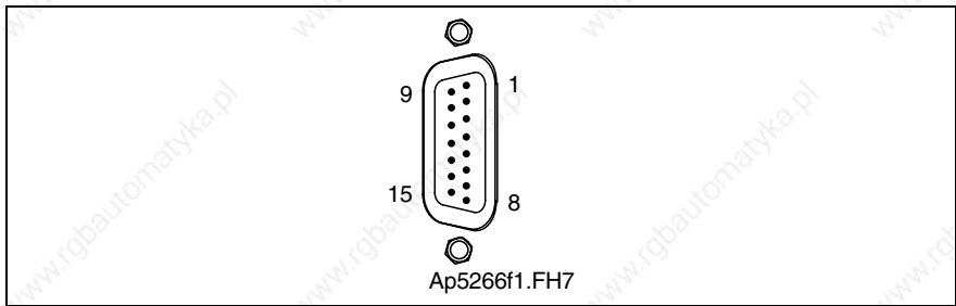
Fig. 4-110: Connector X5
