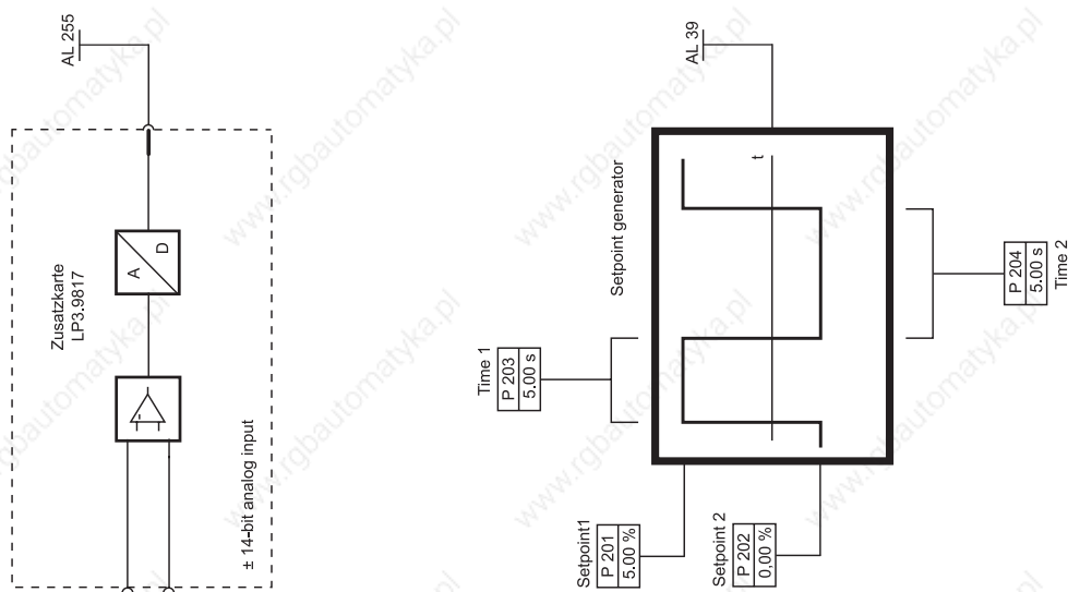
Illustration 37: Function diagram - Setpoints
