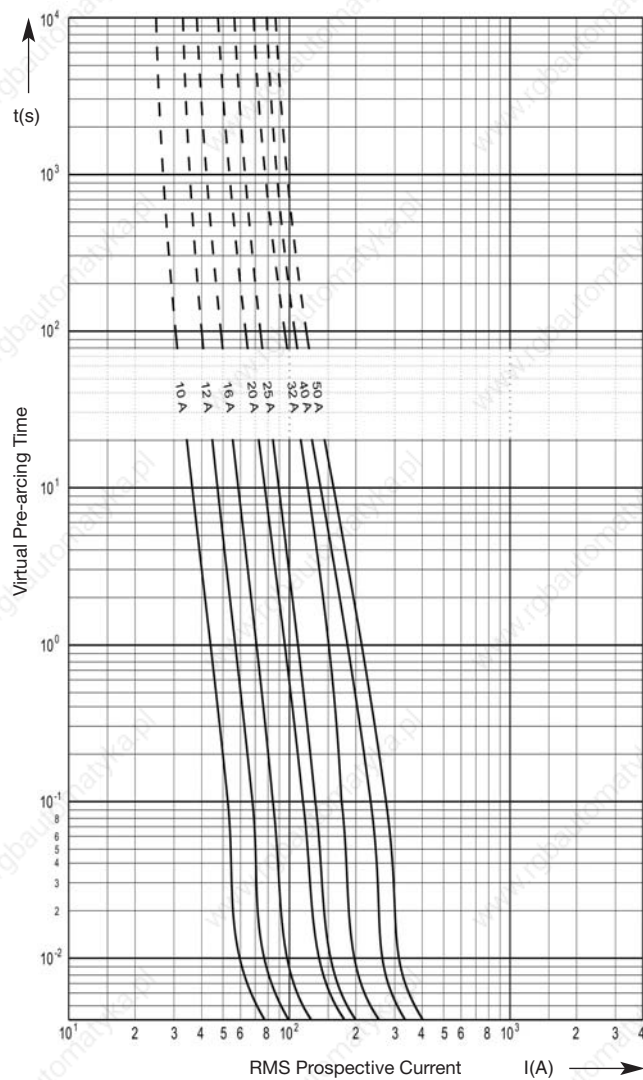
Time-Current Characteristics
