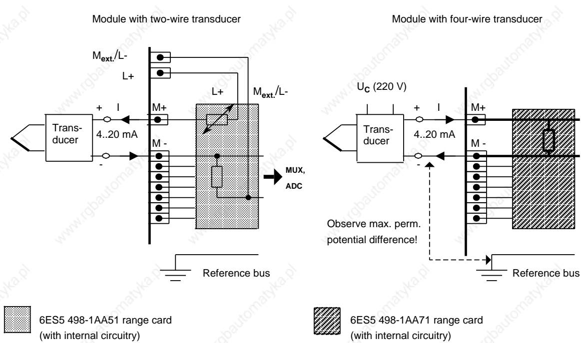
Figure 10-8. Connecting Transducers
