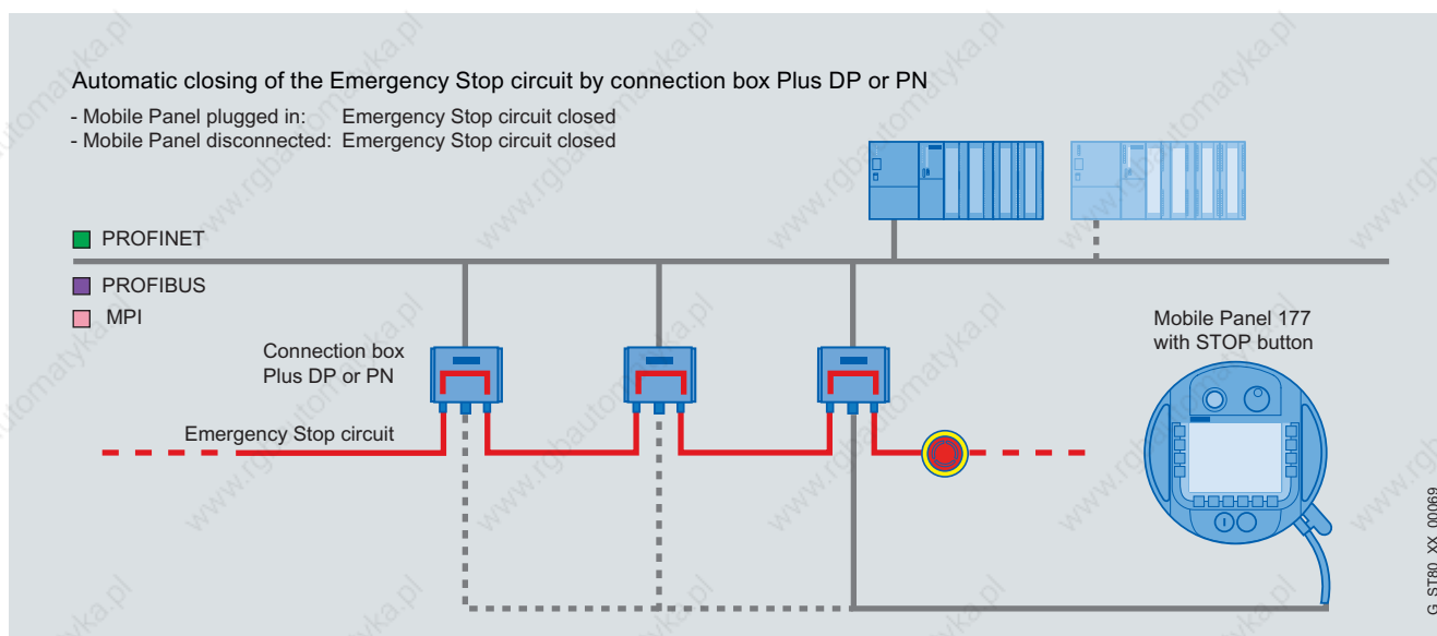
Variable connection to different stations, using the Mobile Panel 177 on the PROFIBUS as an example
