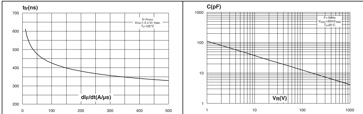
Figure 12. Junction capacitance versus reverse voltage applied (typical values)
