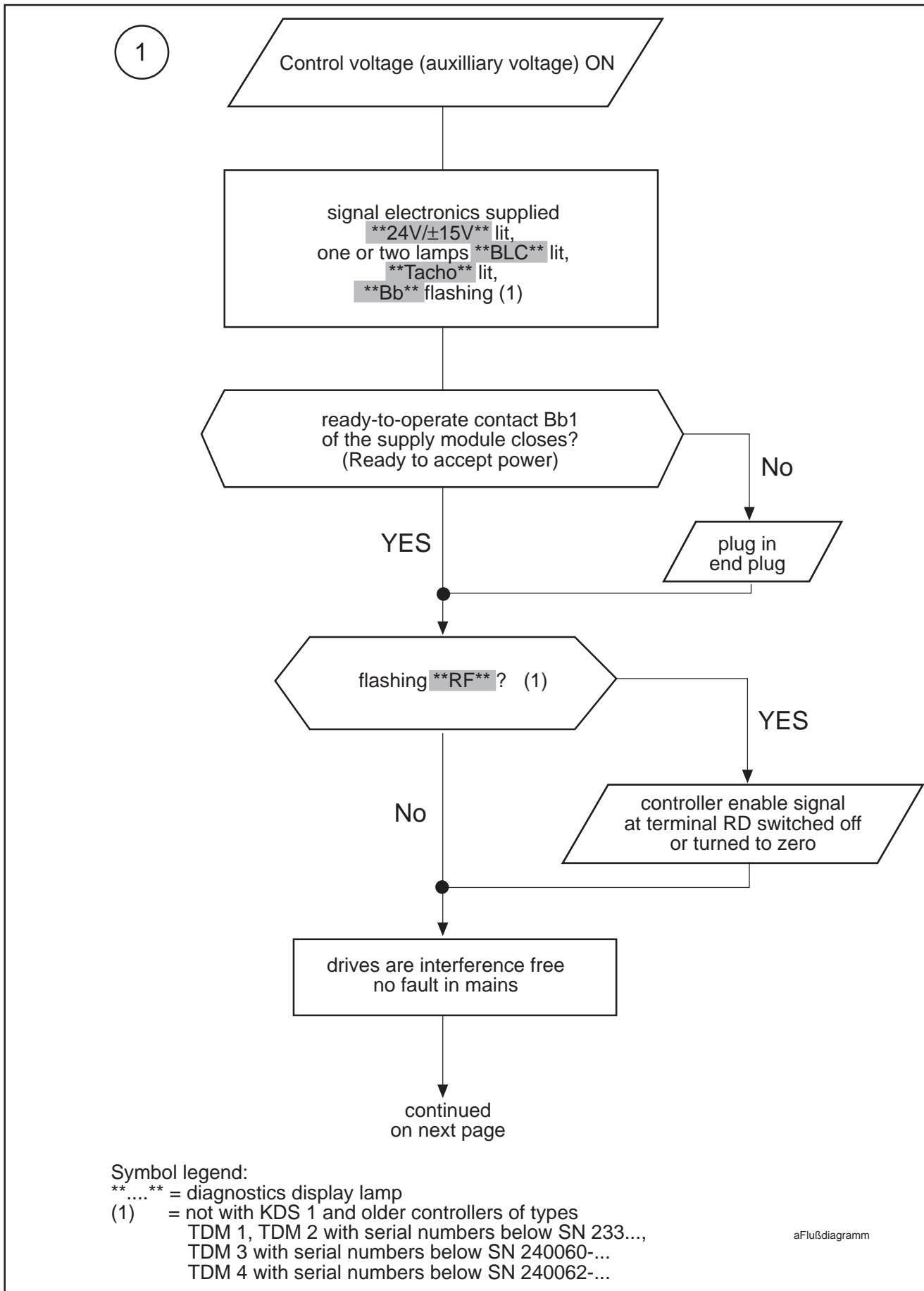
Figure 72: Power-Up Sequence
