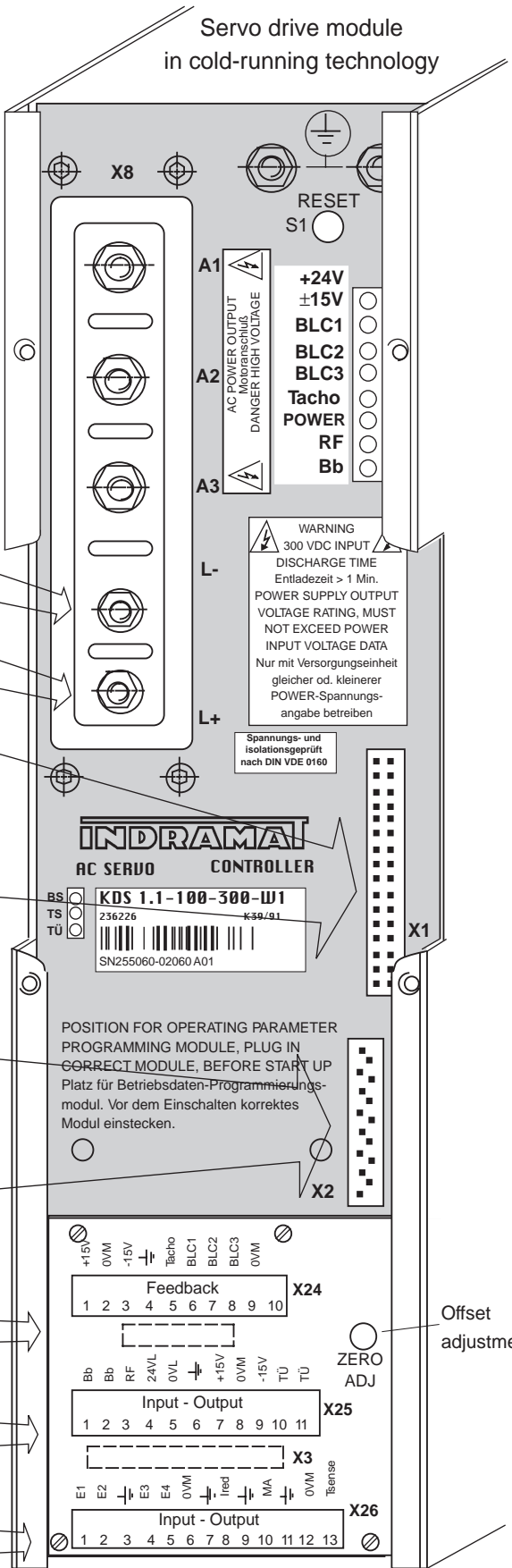
Figure 40: Front view of servo drive module KDS1 with accessories
