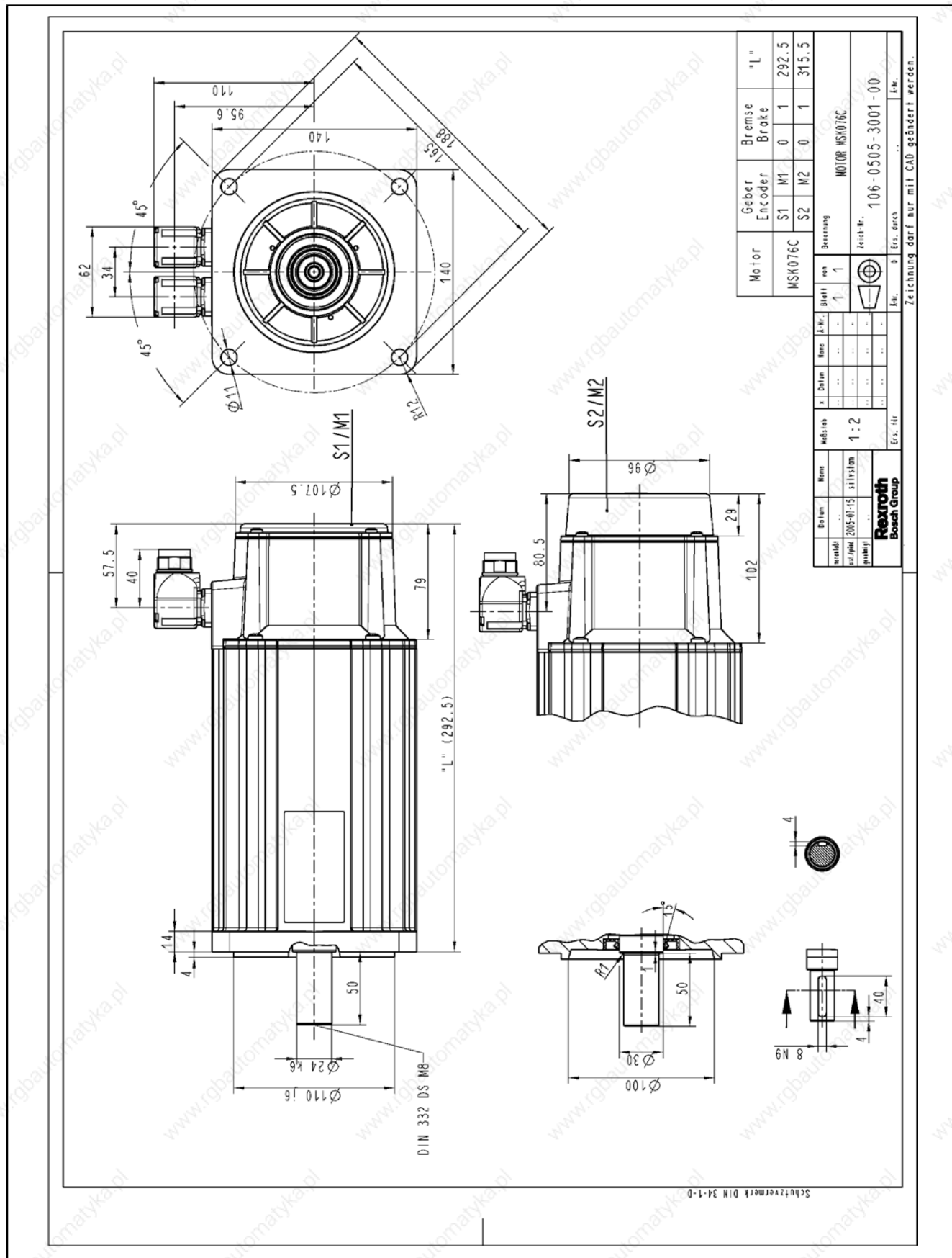
Fig.5-11: MSK076 specification
