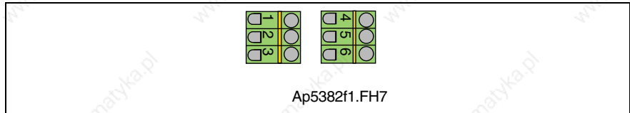
Fig. 5-22: Connector X1
