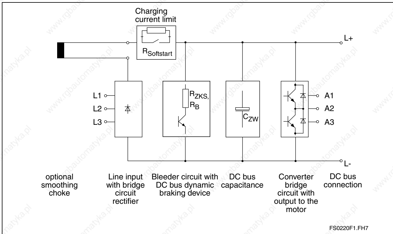
Fig. 4-10: Block diagram of the DKC**.3-200-7-FW power section
