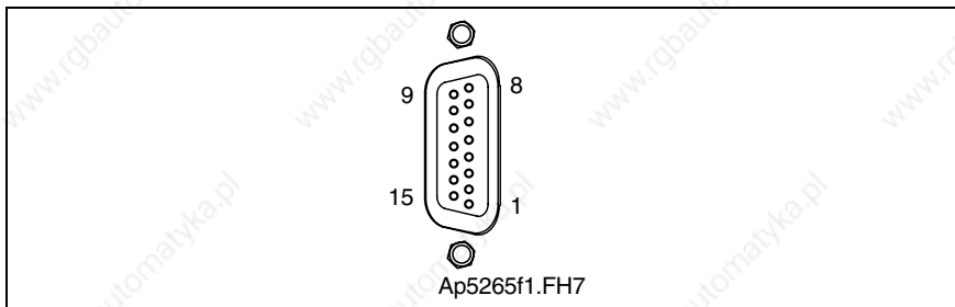
Fig. 5-30: Connector X2
