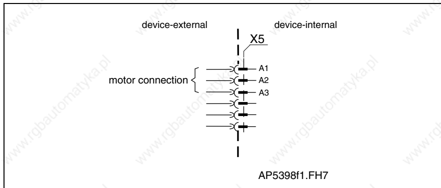
Fig. 5-55: Motor connections
