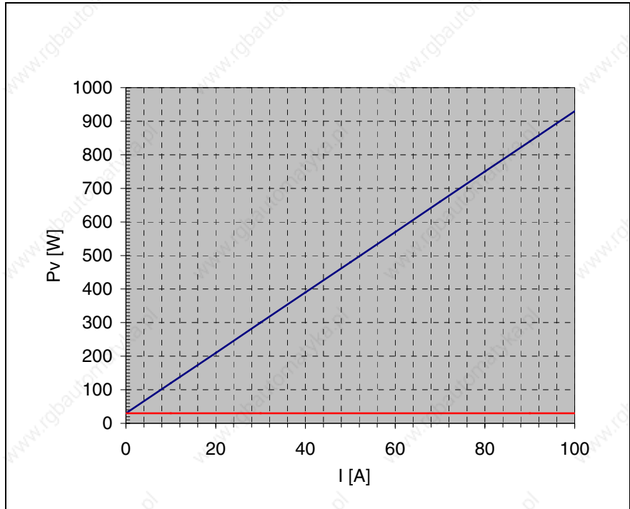
P v : Power dissipation I: Current (Sine threshold value) Fig. 12-8: Determining power dissipation in the control cabinet for each drive controller DKC**.3-200-7-FW without braking resistor power with 4 kHz
