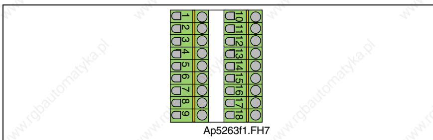
Fig. 4-138: Connector X11
