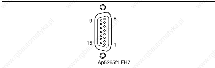
Fig. 5-44: Connector X4
