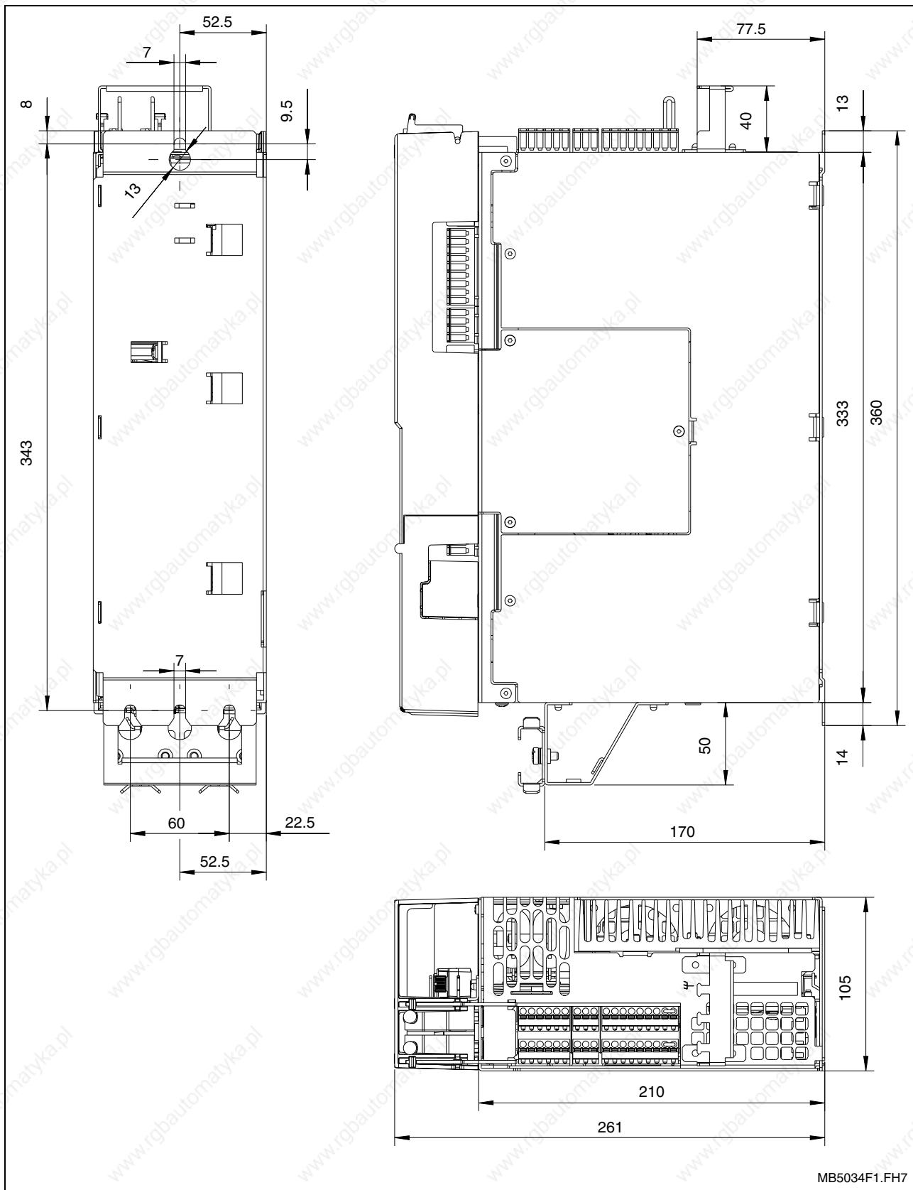
Fig. 4-2: Drive Controller DKC**.3-100-7-FW
