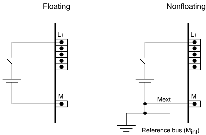
Figure 3-25. Connection to Floating and Nonfloating Modules
