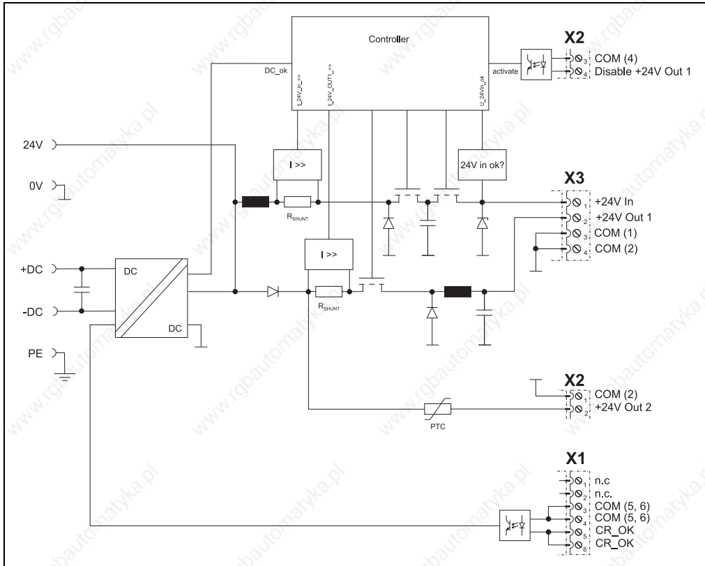
Figure 146: Input/output circuit diagram - 8B0C0320Hx00.00A-1
