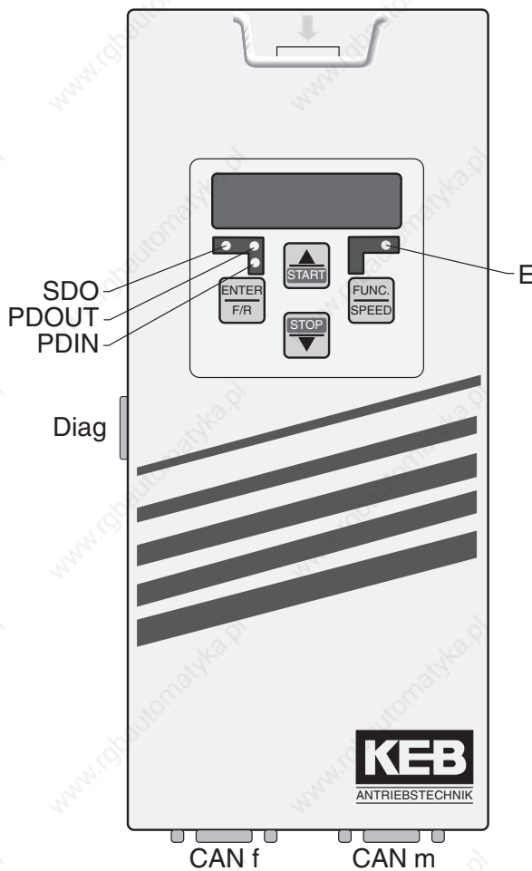
Fig. 11.1.7 CanOpen operator
