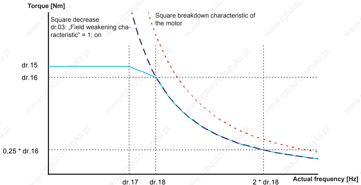
Figure 7.8.2.2 b Field weakening range square reduction
