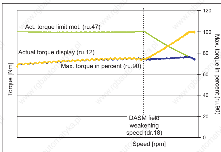
Figure 7.8.6.1 LE.27 = 0
