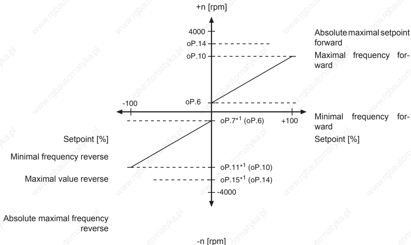
Figure 7.4.5 Setpoint limits
