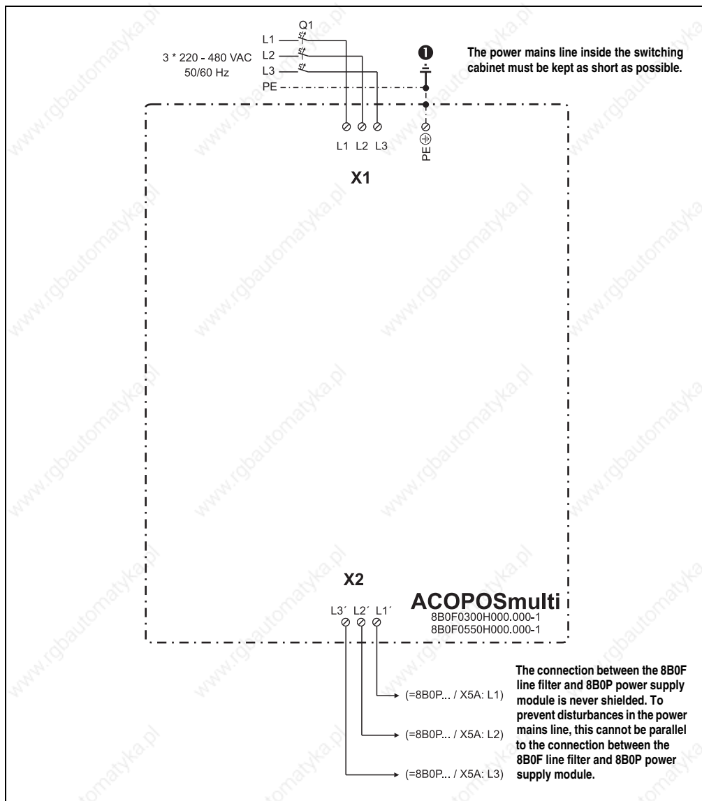
Figure 102: Ground connections and shield connections for 8B0F line filter
