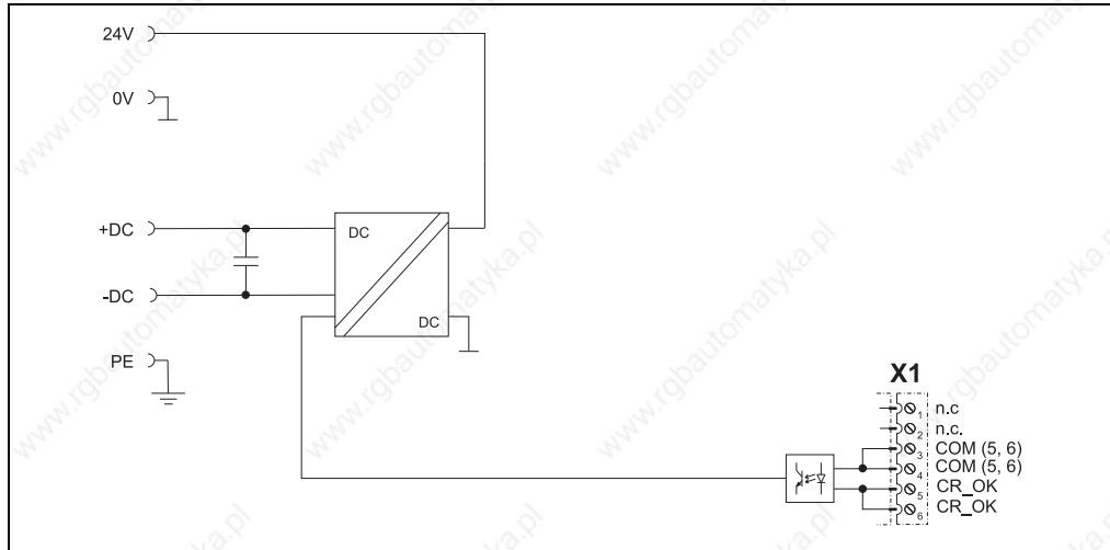
Figure 140: Input/output circuit diagram - 8B0C0160Hx00.000-1, 8B0C0320Hx00.000-1
