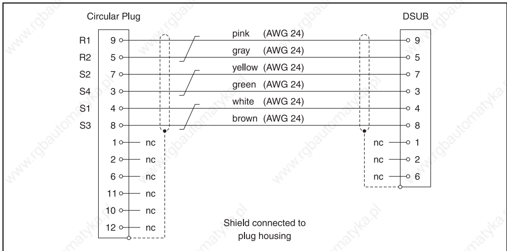
Figure 185: Cable schematic - 8BCR resolver cables
