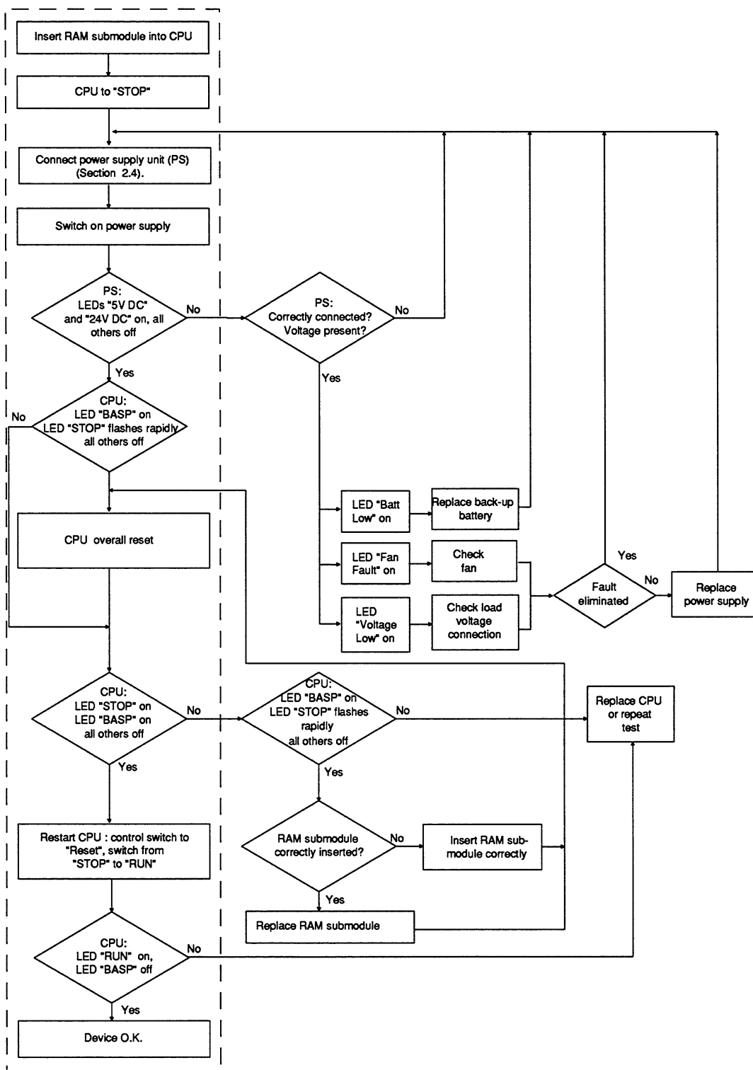
Fig. 15 Starting up
