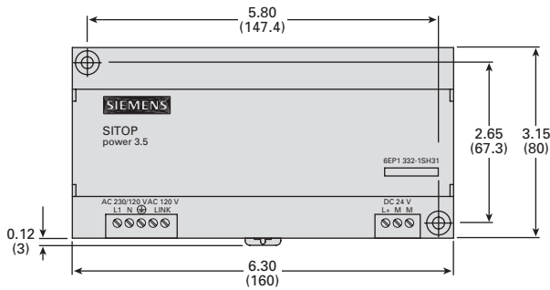
6EP1332-1SH31, DC 24V/3.5A
