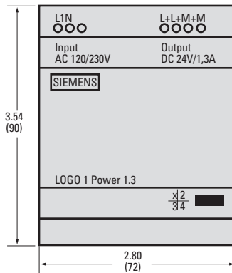
6EP1331-1SH01, DC 24V/1.3A
