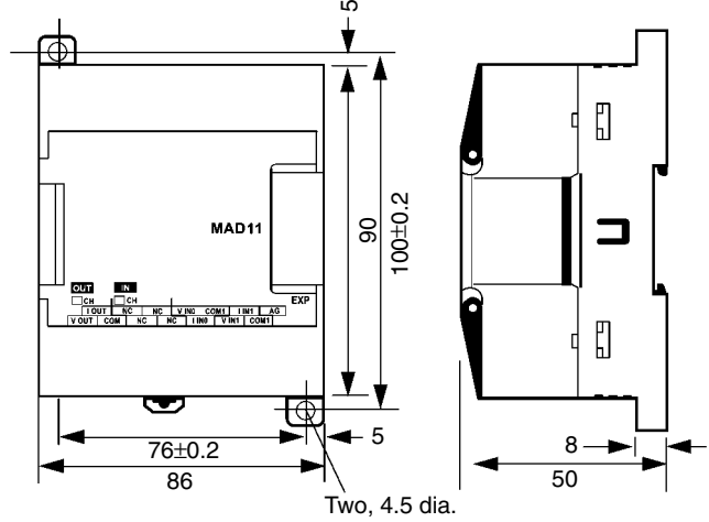
CPM1A-MAD11
