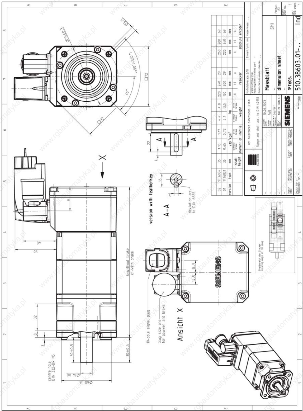
Figure 5-2 1FT603□-□A□DQ
