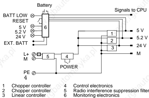
Block diagram
