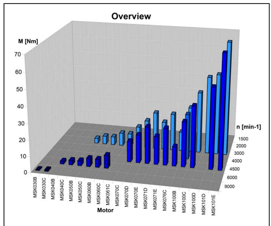
Fig. 1-1: MSK power graduation
