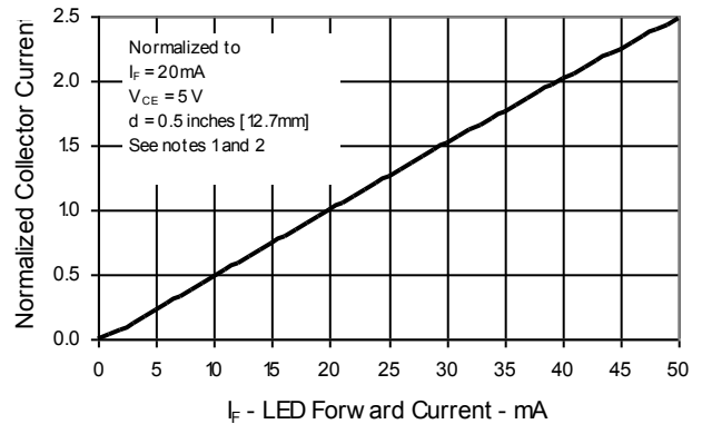
Normalized Collector Current Vs LED Forward Current
