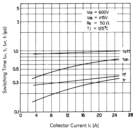
Switching Time
