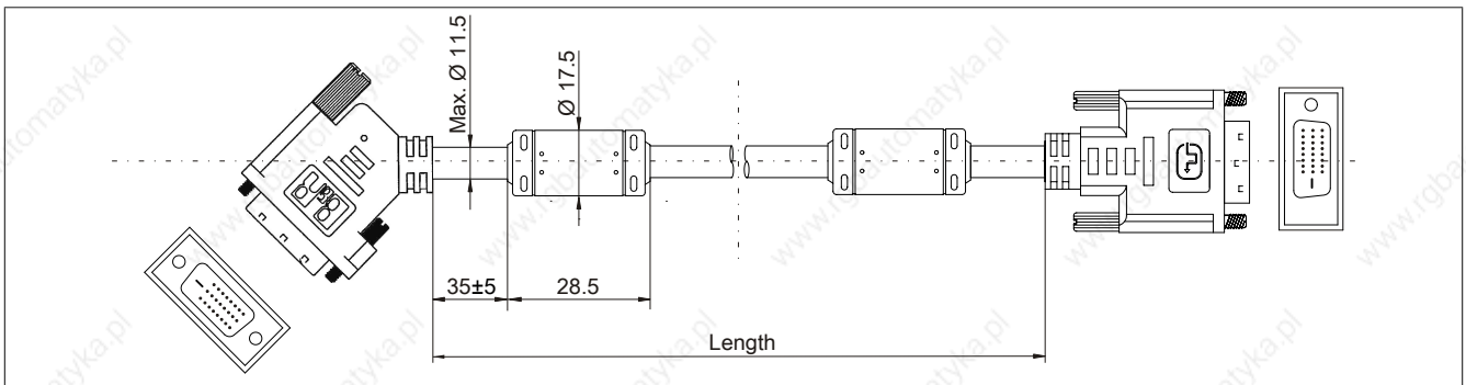
Figure 212: 5CASDL.0xxx-01 - Dimensions
