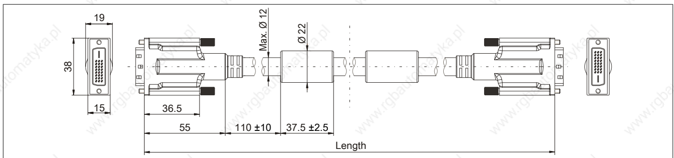
Figure 215: 5CASDL.0xxx-03 - Dimensions
