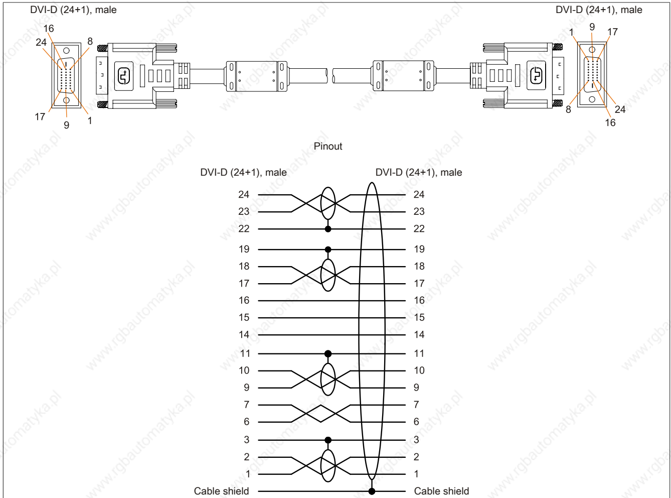
Figure 207: 5CADVI.0xxx-00 - Pinout
