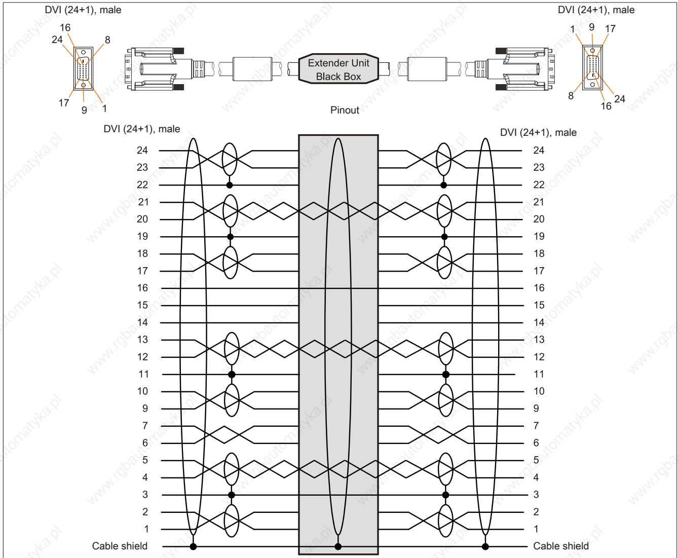
Figure 219: 5CASDL.0xx0-13 - Pinout
