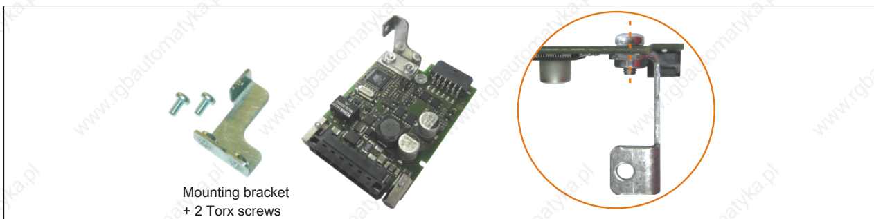
Figure 270: Installing the mounting bracket
