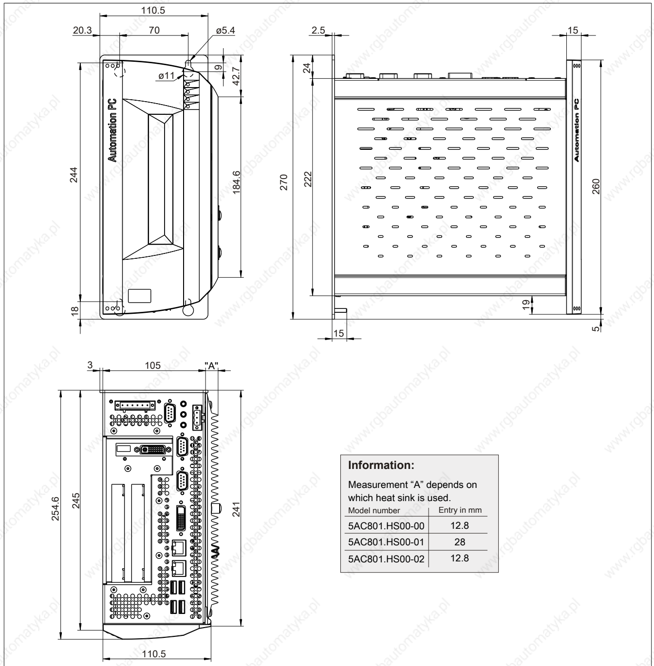
Figure 25: 5PC810.SX02-00 - Dimensions
