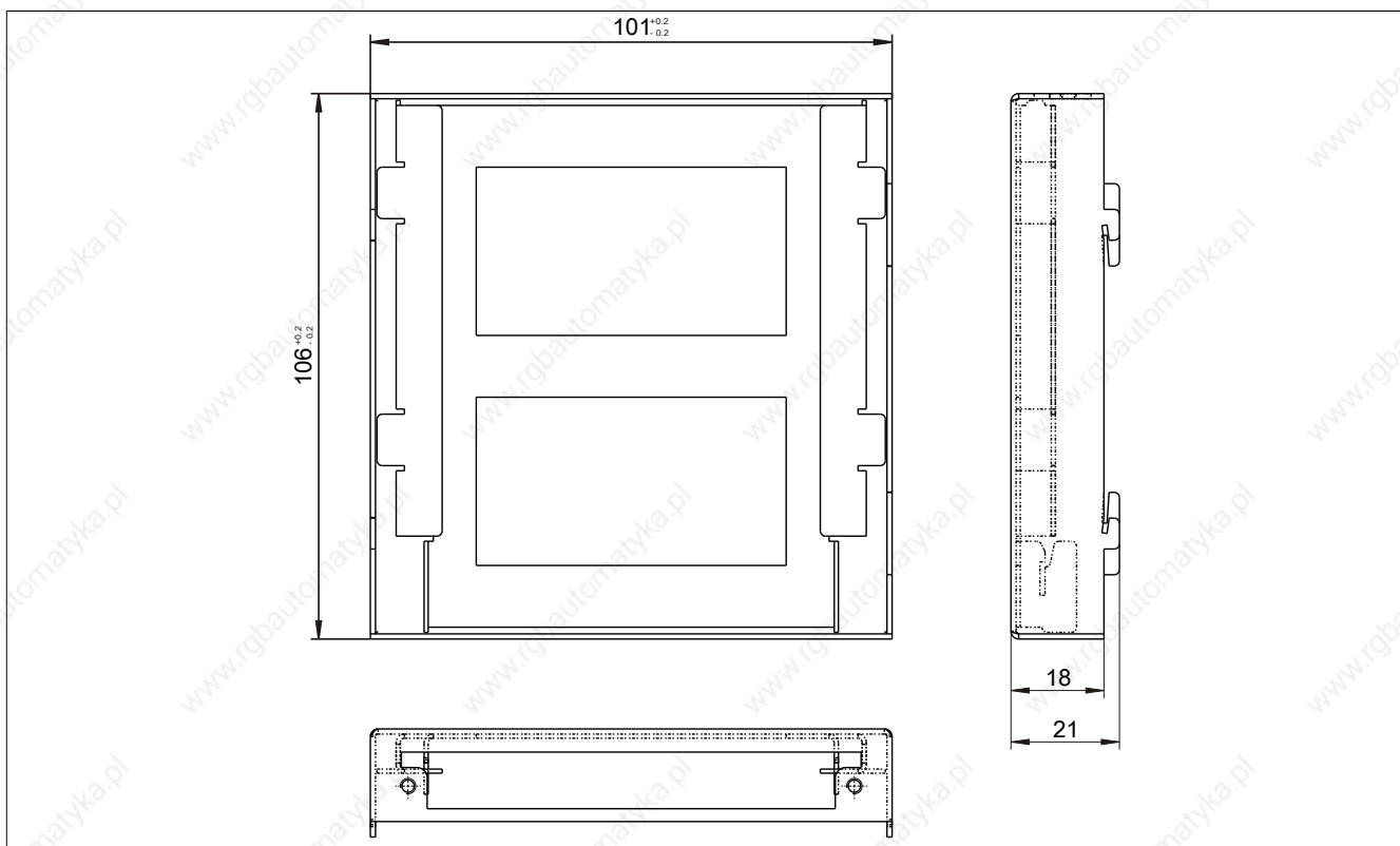
Figure 224: 5AC801.FRAM-00 - Dimensions
