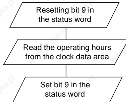
Figure 13-3. Procedure for Reading the Operating Hours Counter
