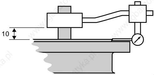
CONCENTRICITY OF SPIGOT AND SHAFT
