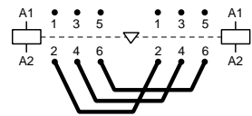
BES110 connection diagram
