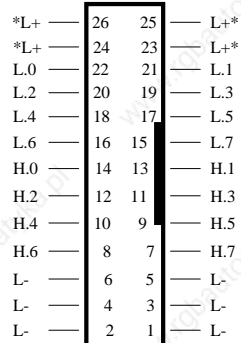
connector strip on DEA-BG0X
