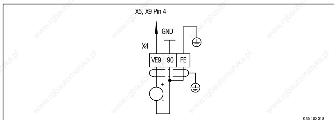
FIG 4-17 Connection of the incremental encoder supply
