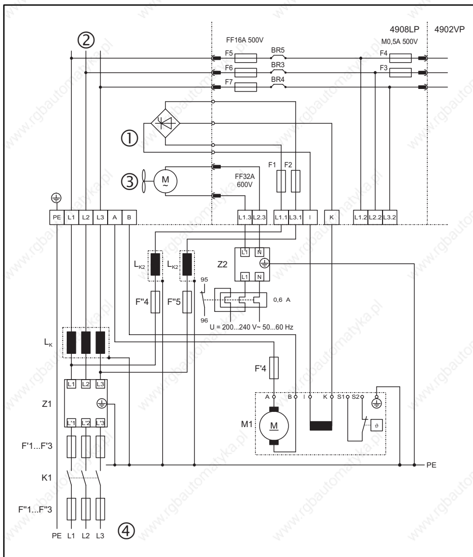
FIG 4-4 Power connection of controllers 4X08 to 4X09
