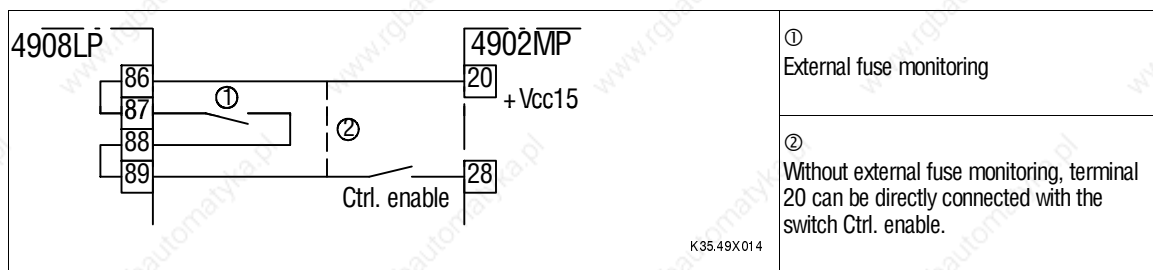
FIG 4-13 4808...4809 and 4908...4909
