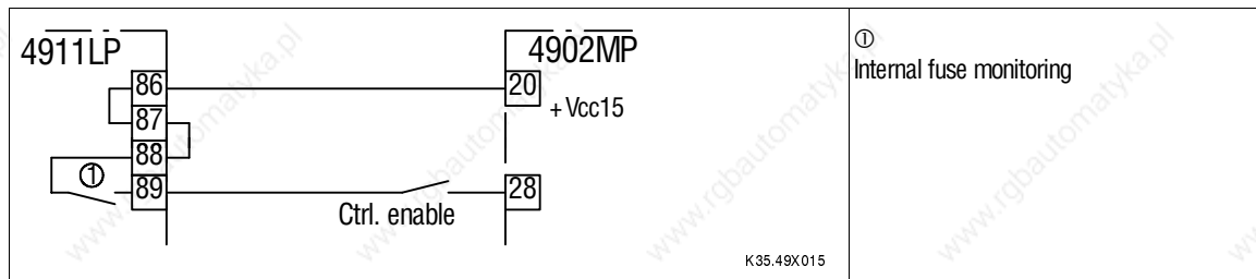
FIG 4-14 4811...4813 and 4911...4913
