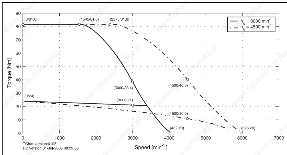
Figure 43: Speed - torque characteristic curve for 8LSA65.eennnffgg-0
