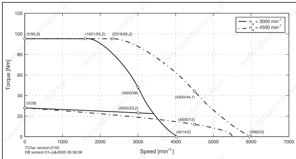
Figure 44: Speed - torque characteristic curve for 8LSA66.eennnffgg-0
