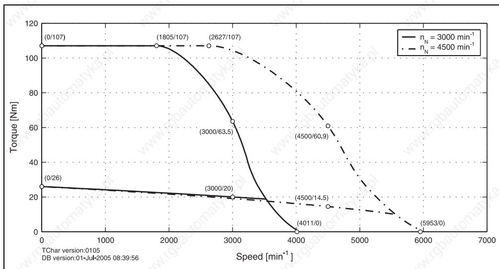
Figure 49: Speed - torque characteristic curve for 8LSA73.eennffgg-0
