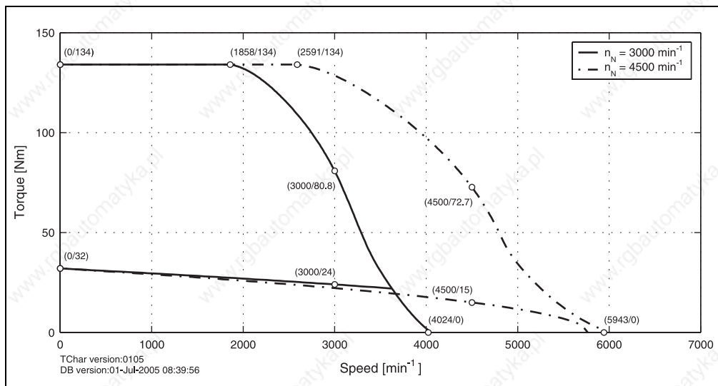
Figure 50: Speed - torque characteristic curve for 8LSA74.eennffgg-0
