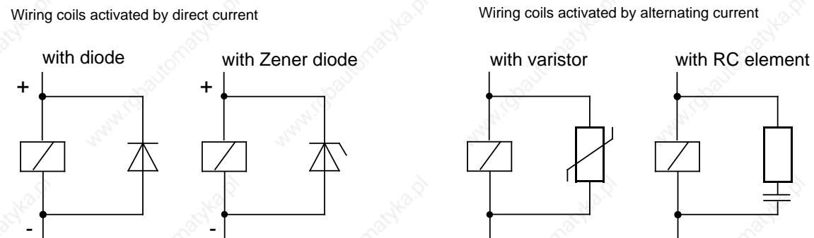
Figure 3-27. Wiring Coils
