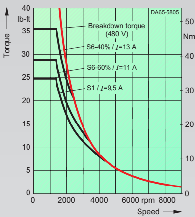
1PH7103-2.D...-.... max. breakdown torque: 53 lb-ft/73 Nm
