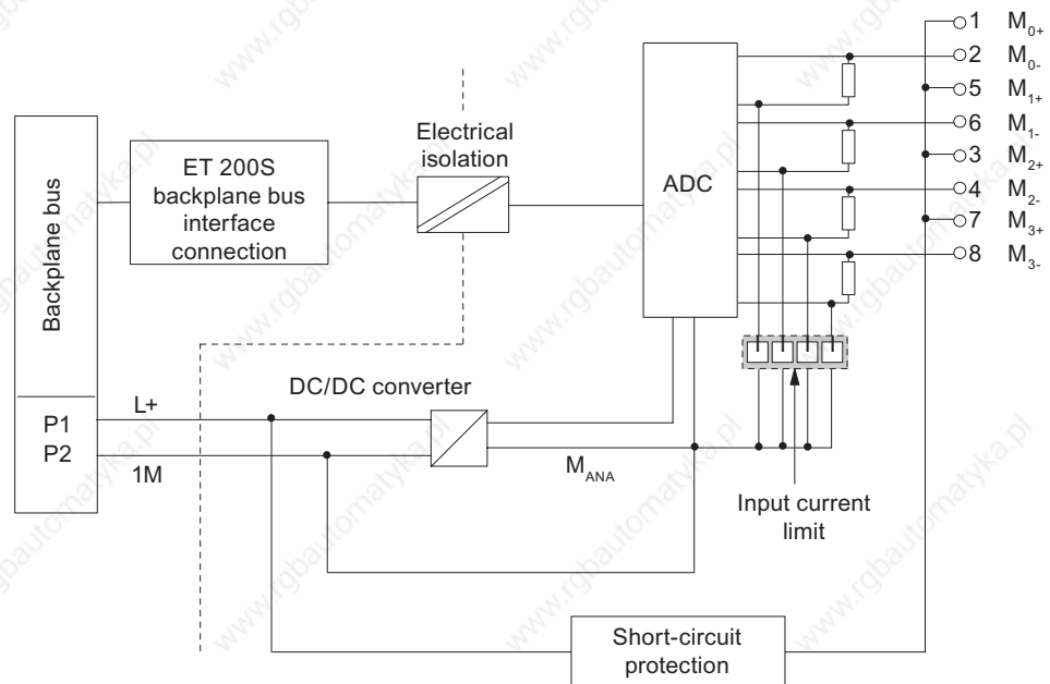
Figure 4-10 Block diagram of the 4AI | 2WIRE Standard
