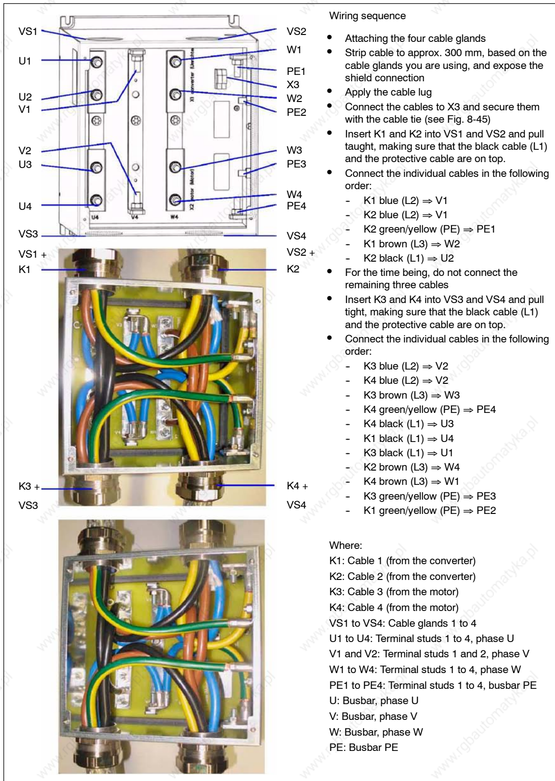
Fig. 8-43 Connection of internal cable routing and VPM 200 Dynamik
