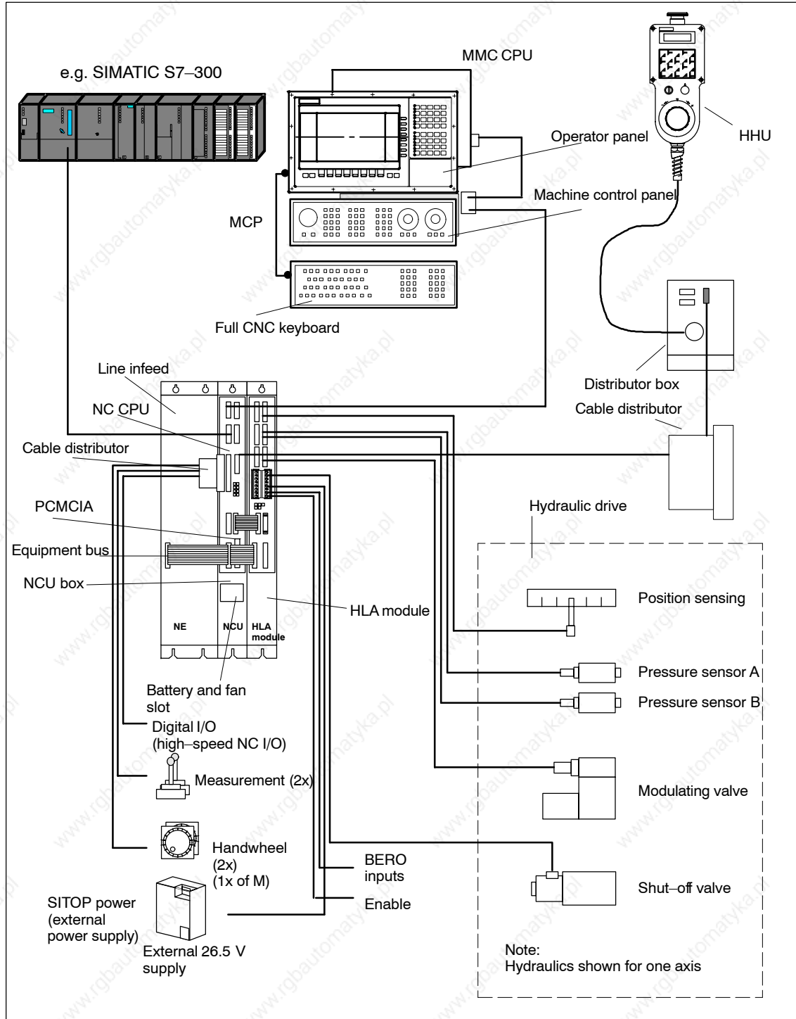
Fig. 5-9 System components
