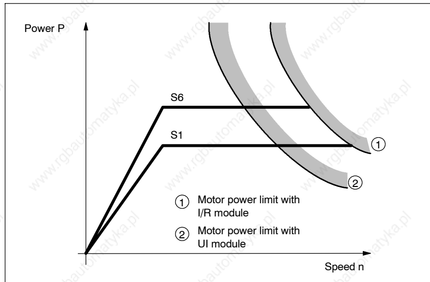
Fig. 4-10 Speed/power graph
