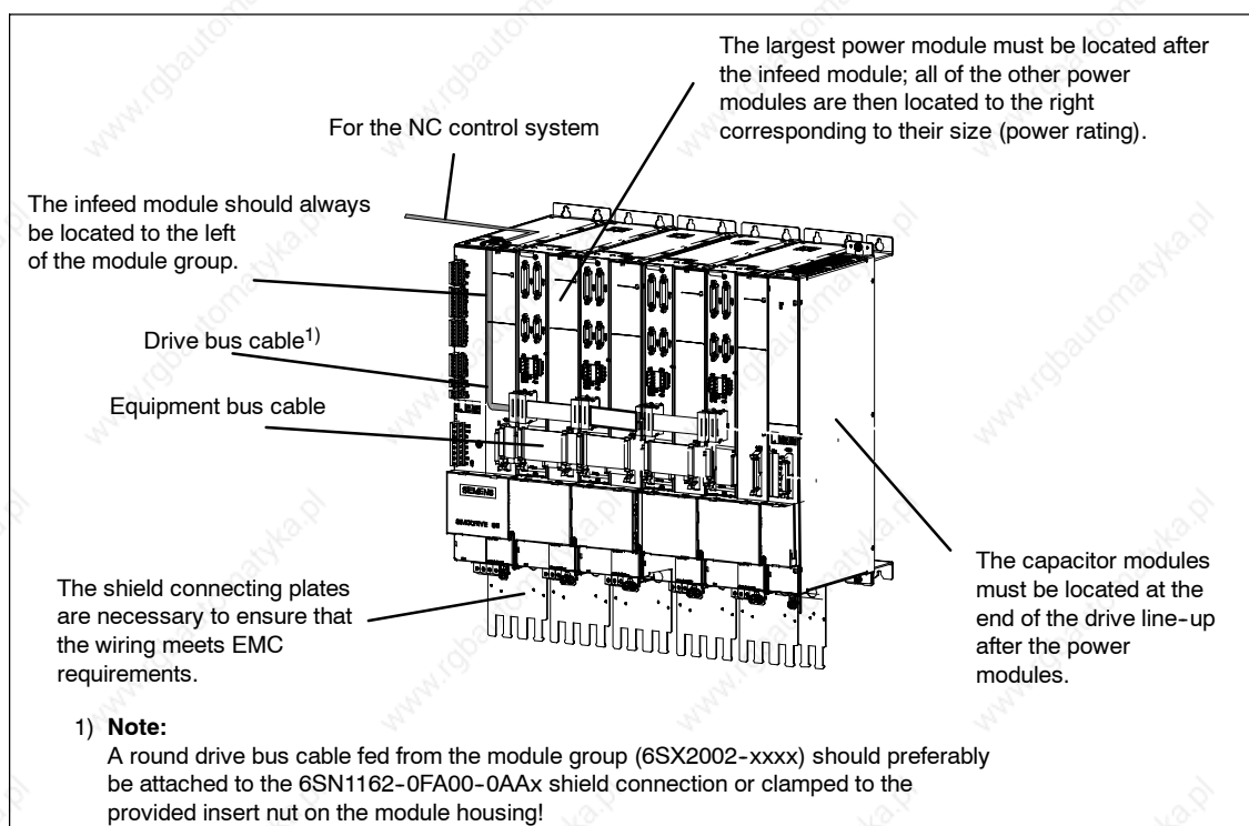
Fig. 2-1 Connection example
