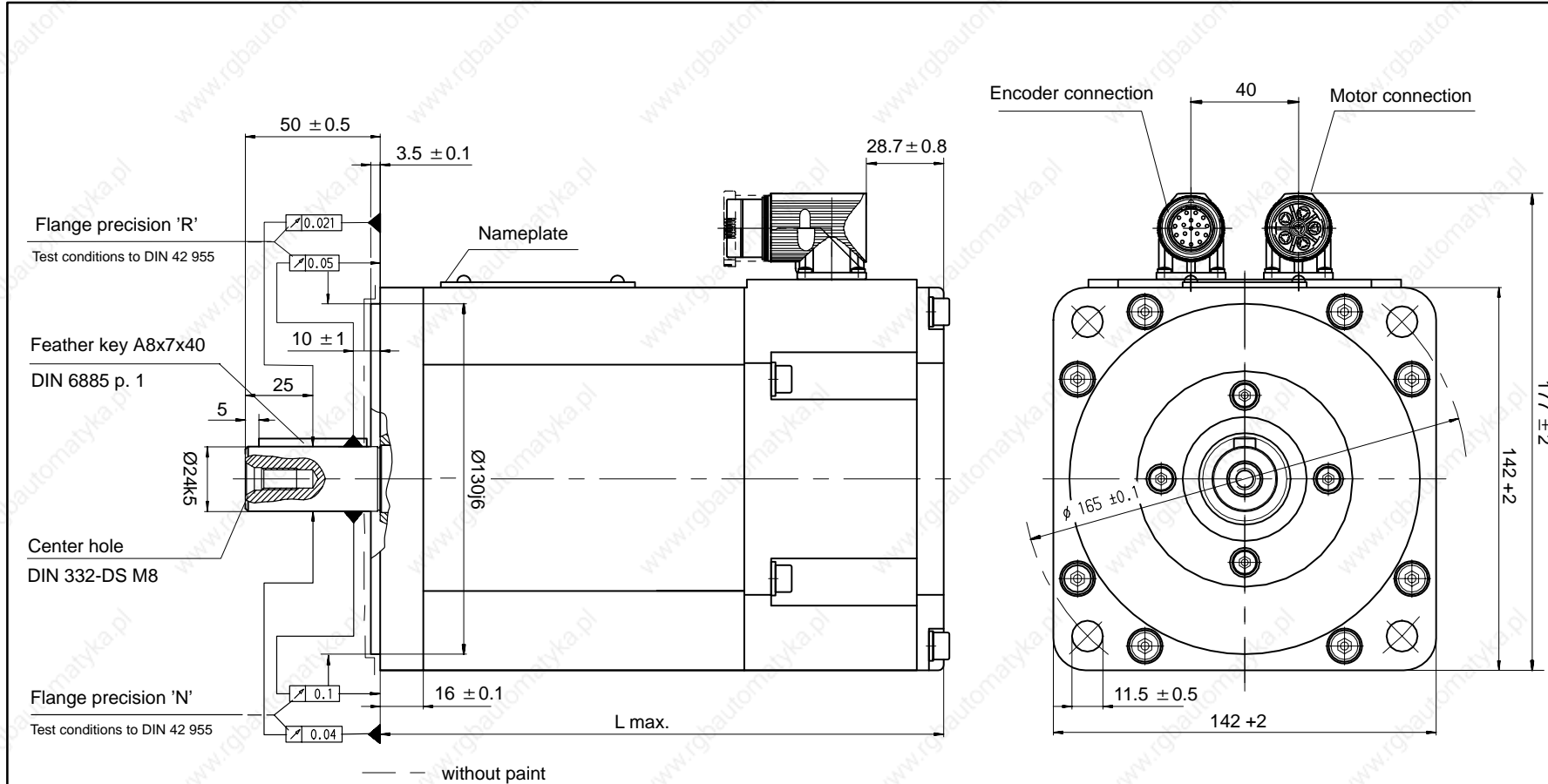
Motor type SF(R)-A4... .015/.030
