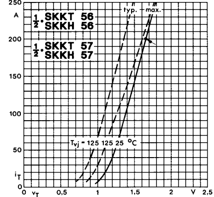
Fig. 8 On-state characteristics
