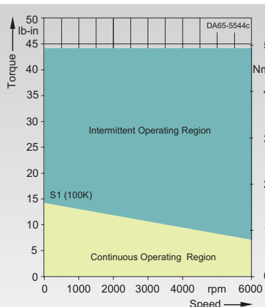
1FK6040-6AK71-1...
