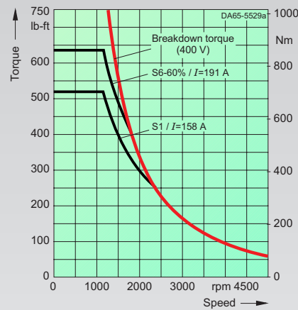
1PL6186-4.D. max. breakdown torque: 871 lb-ft/1181 Nm
