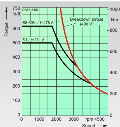
1PL6186-4.F. max. breakdown torque: 1210 lb-ft/1640 Nm
