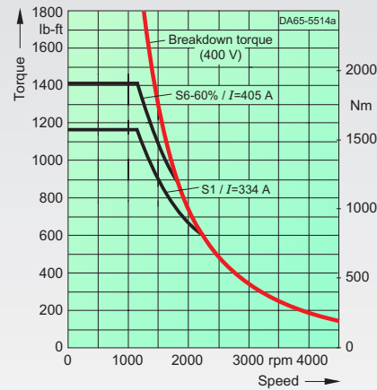
1PL6228-4.D. max. breakdown torque: 2127 lb-ft/2884 Nm
