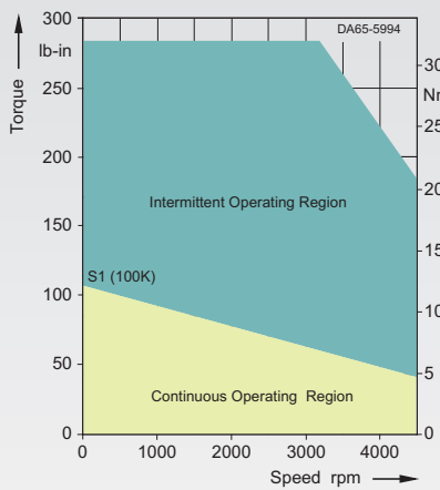
1FK6064-7AH71-1...
