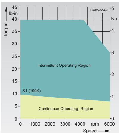
1FK6032-6AK71-1...
