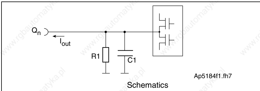
Fig. 4-69: Control outputs
