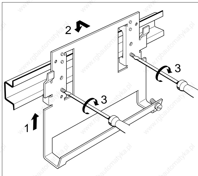
Figure 3-5 Mounting the Shield Connecting Element on the Standard Sectional Rail
