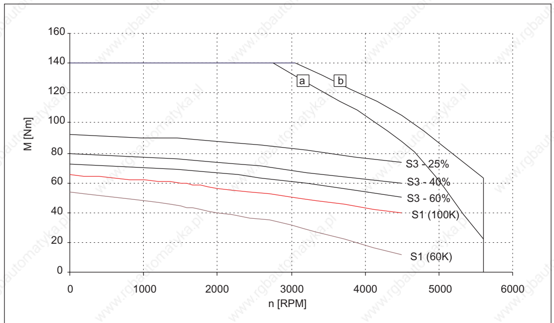
Figure 3-62 Speed-torque diagram 1FT6105-8SH7□
