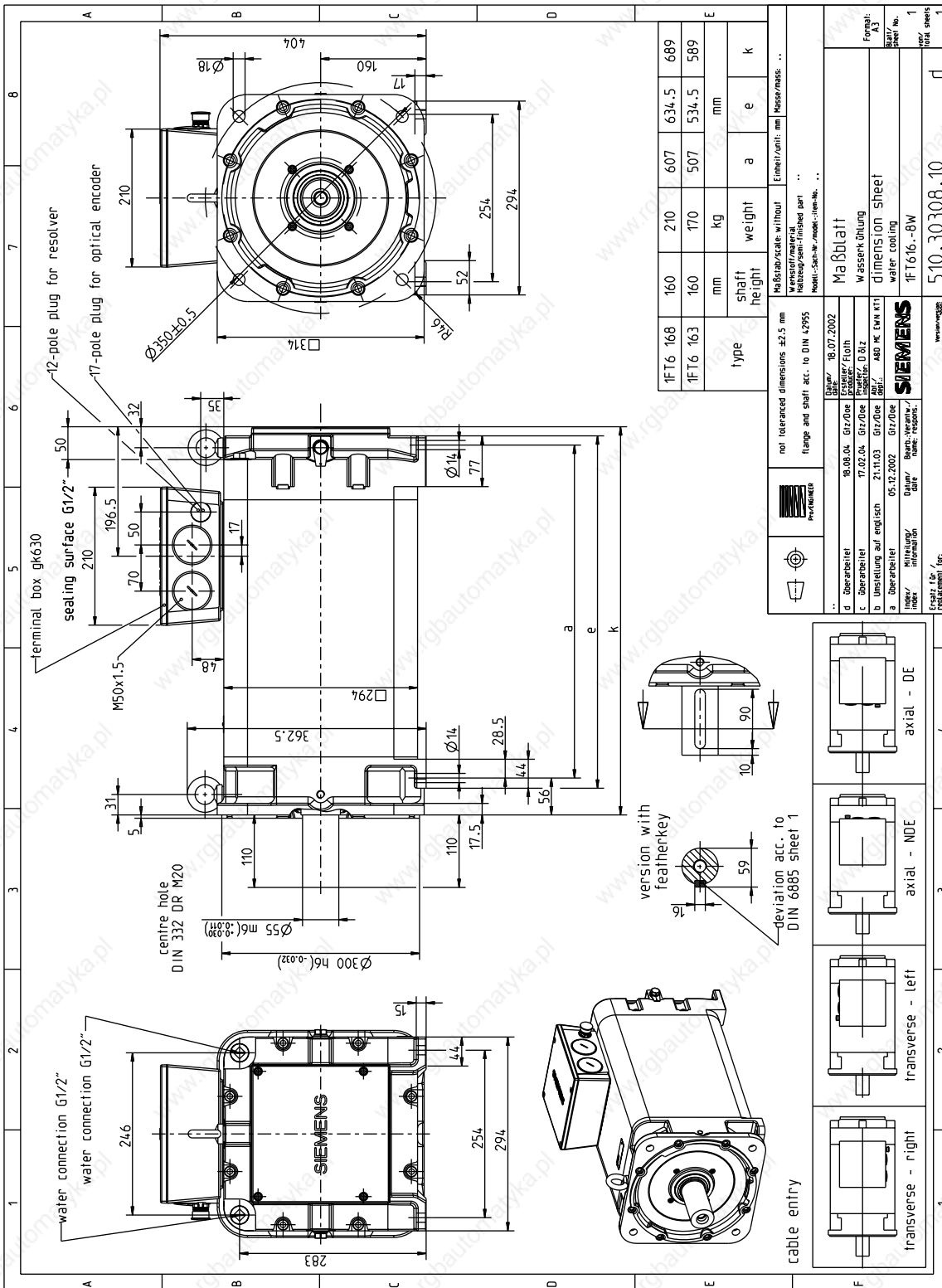
Figure 5-41 1FT616x-8Wx76-5xxx
