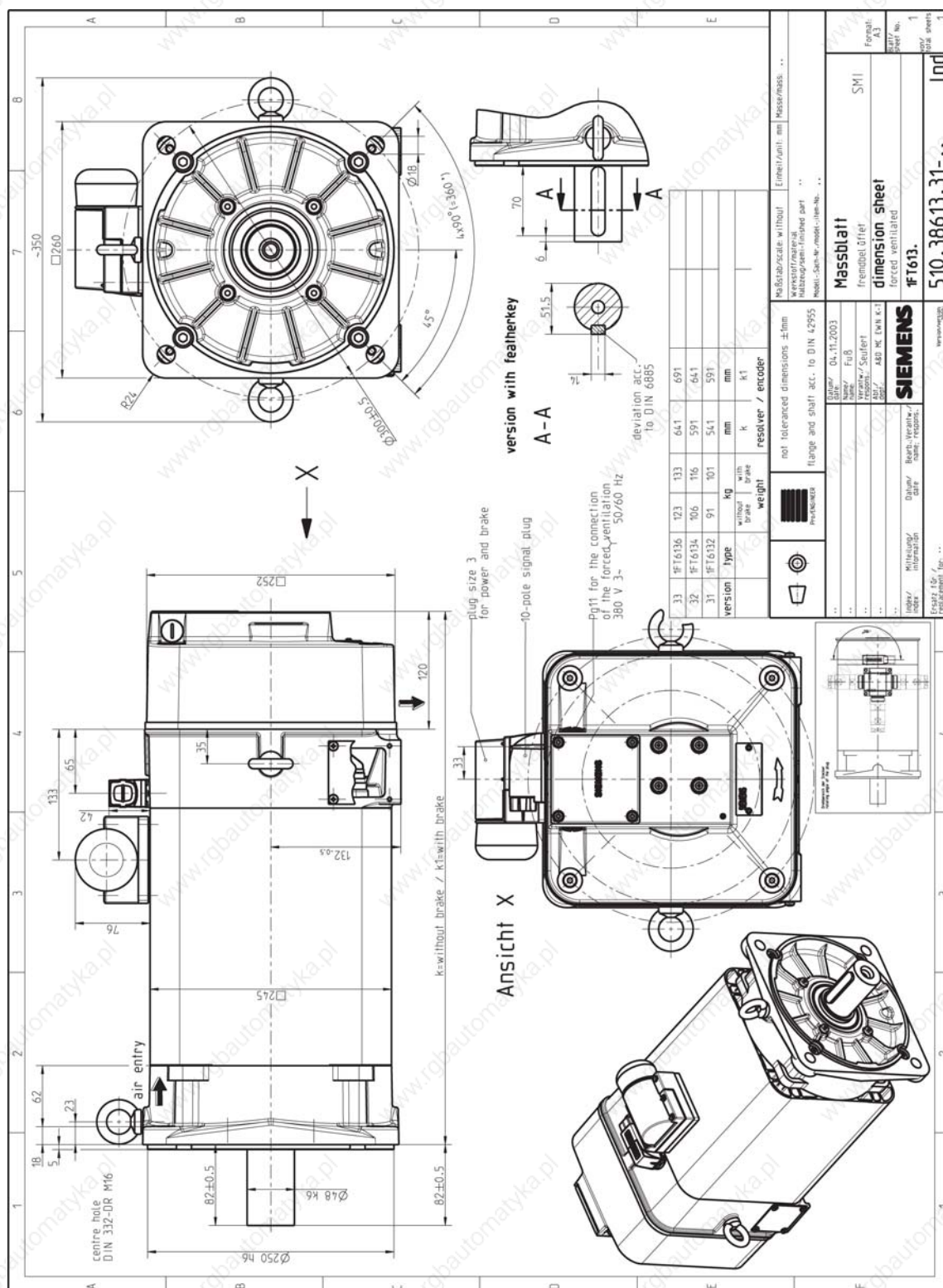
Figure 5-11 1FT613□-□S□plug□DQ
