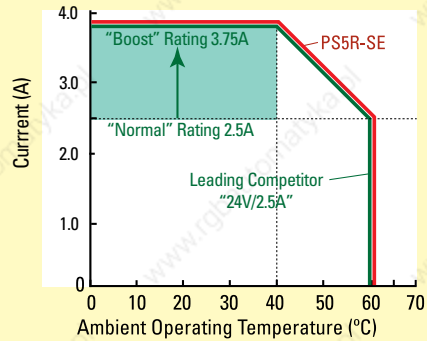
PS5R-SE 90W/3.75A/24V DC versus the Leading Competitor Standard derating curve (operating temperature vs. output current)
